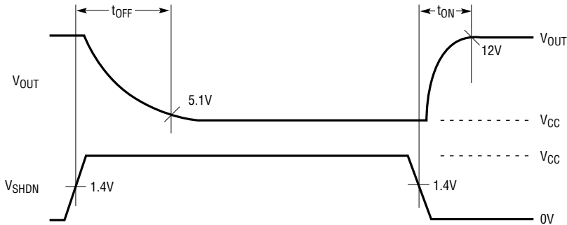
Figure 1. Timing Diagram
