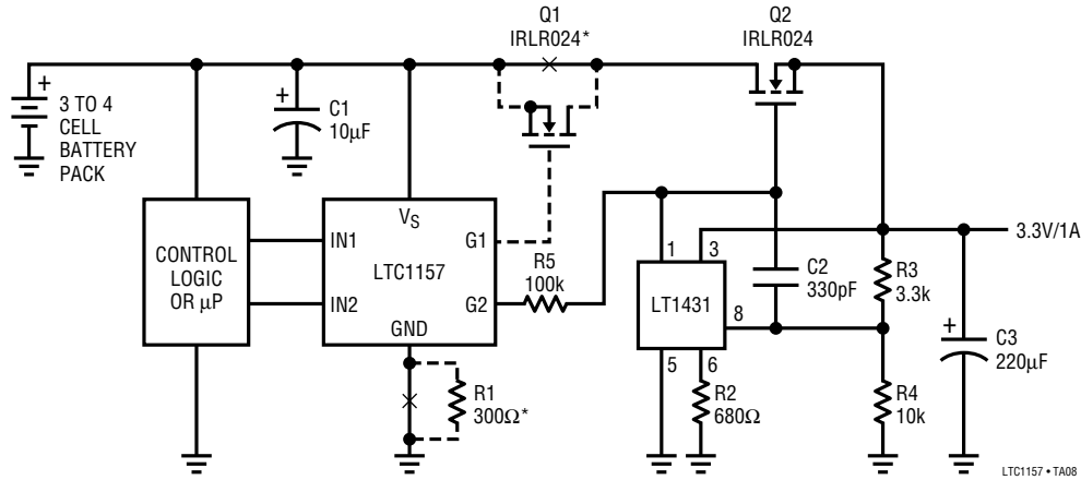
3.3V Ultra Low Voltage Drop Regulator with Optional Reverse Battery Protection and 3µA Standby Current
