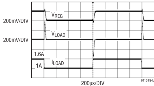
Figure 24c. Capacitor C_{COMP} Compensates for the LT6110 in the Regulator's Loop
