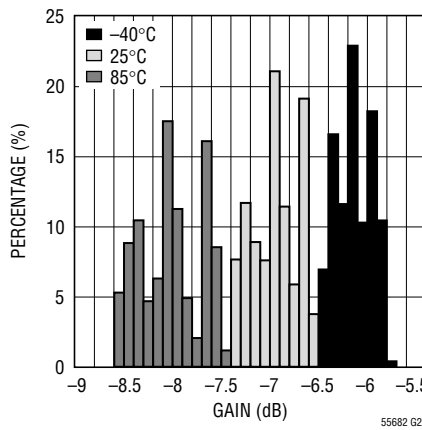
Gain Distribution
