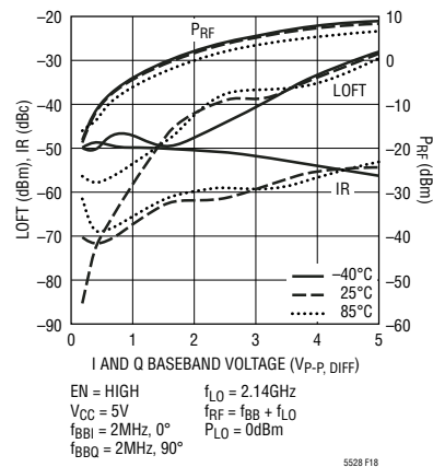
Figure 18: LO Feed-Through and Image Rejection vs Baseband Drive Voltage after Calibration at 25°C
