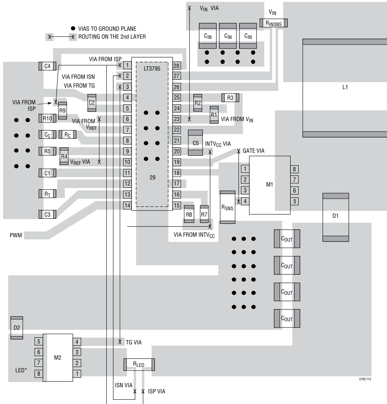
COMPONENT DESIGNATIONS REFER TO PAGE 23 CIRCUIT
