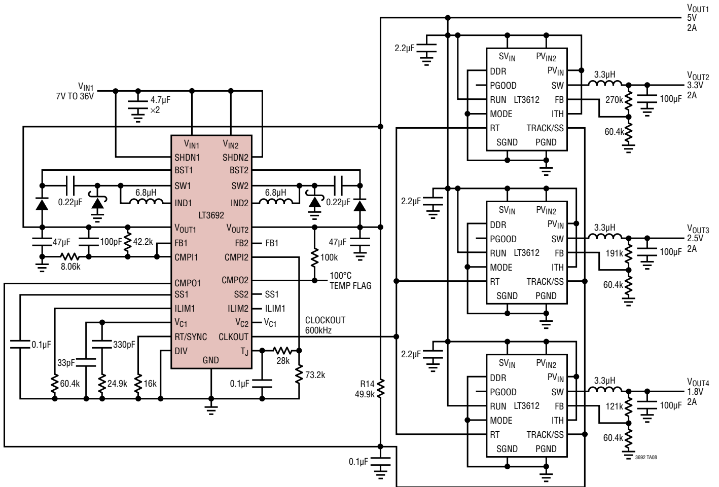
5V, 3.3V, 2.5V, 1.8V Synchronized Quad Output
