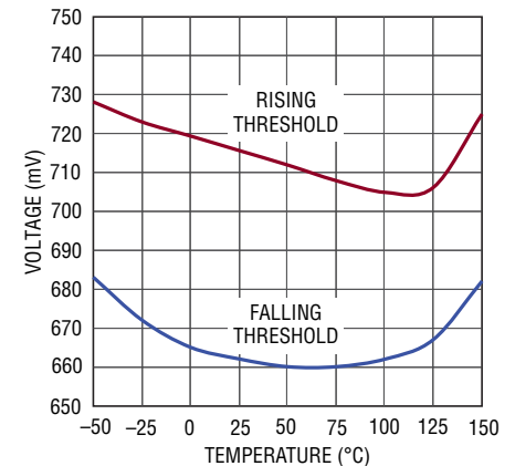
Comparator Thresholds vs Temperature
