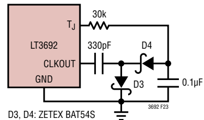
Figure 22. Circuit to Generate the Negative Voltage Rail to Extend the T J Pin Operating Range
