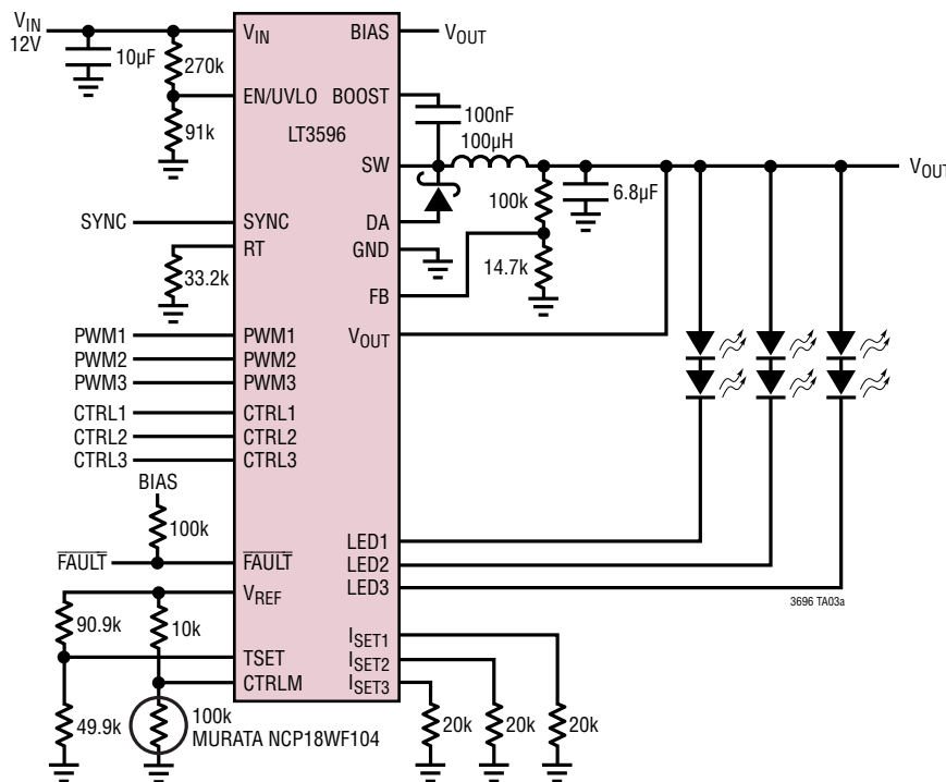
12V 1MHz Step-Down 100mA Single Pixel R-G-B Driver
