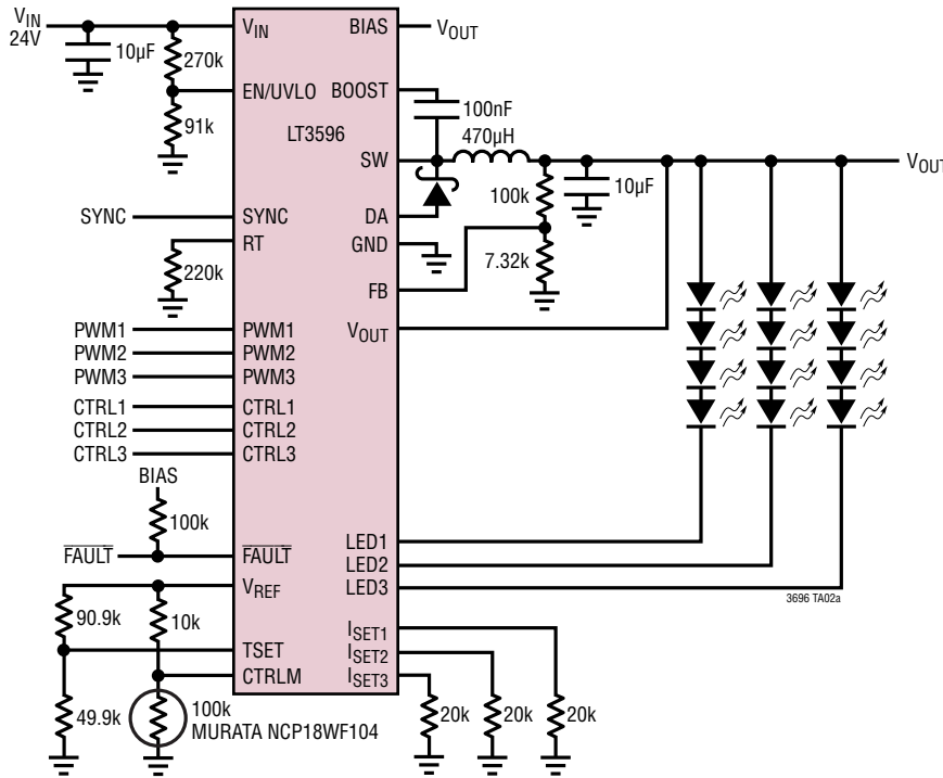
24V 200kHz Step-Down 4W, 100mA LED Driver
