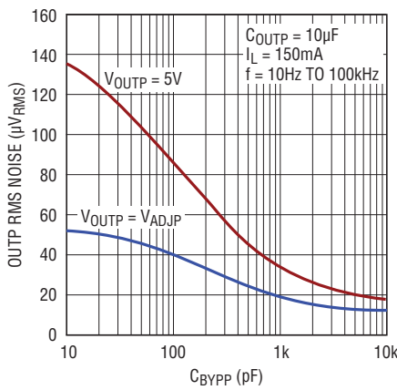
OUTP RMS Noise vs Bypass Capacitor
