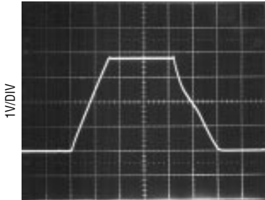
A_V = 1 100\mu s/DIV C_L = 12pF INPUT PULSE = 0V TO 3.8V LT2178/79 • TPC14
