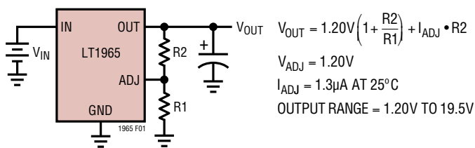
Figure 1. Adjustable Operation
