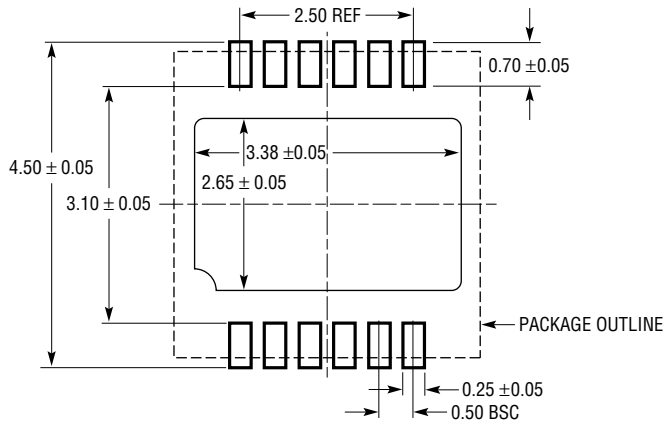
DF Package 12-Lead Plastic DFN (4mm × 4mm) (Reference LTC DWG # 05-08-1773 Rev 0)
