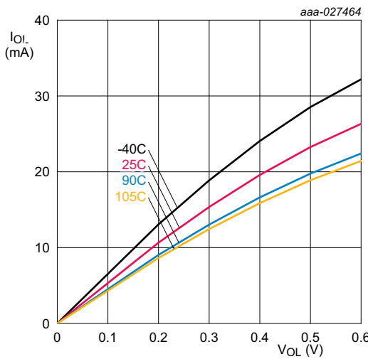
Fig 24. I 2 C-bus pins (high current sink): Typical LOW-level output current I_{OL} versus LOW-level output voltage V_{OL}
