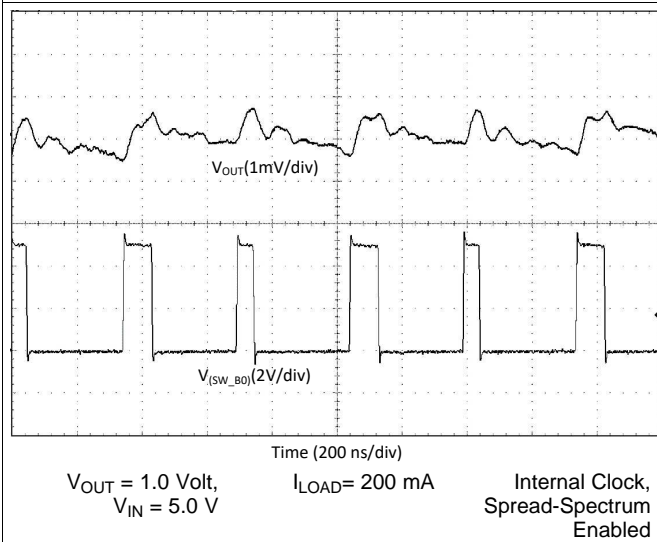
Figure 30. Output Voltage Ripple, Forced-PWM Mode
