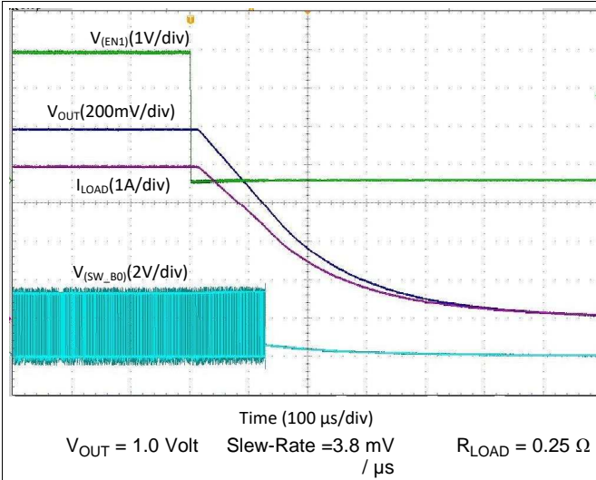
Figure 28. Shutdown With EN1, Forced PWM
