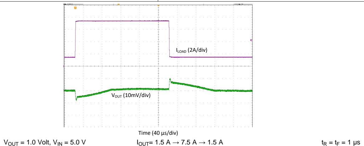
Figure 32. Transient Load Step Response, Forced-PWM Mode
