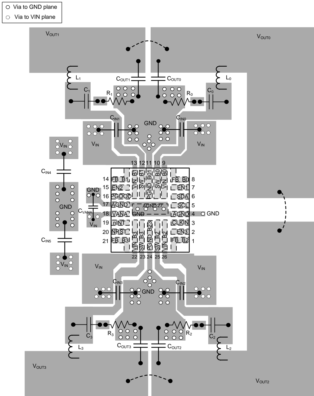
Figure 33. Board Layout
