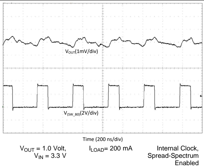
Figure 29. Output Voltage Ripple, Forced-PWM Mode
