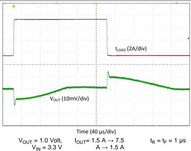
Figure 31. Transient Load Step Response, Forced-PWM Mode
