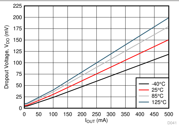
Figure 6-44. LP5912-1.8 Dropout Voltage ( V_{DO} ) vs I_{OUT}
