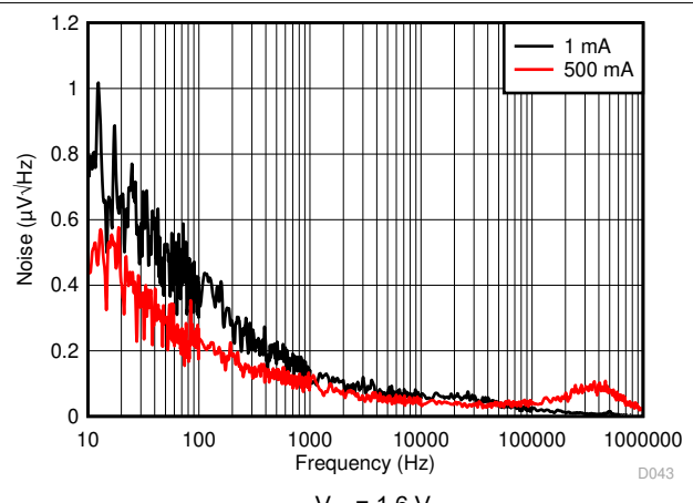
Figure 6-46. LP5912-0.9 Noise vs Frequency
