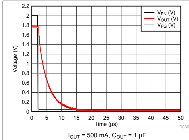
Figure 6-43. LP5912-1.8 V_{OUT} vs V_{EN(OFF)}
