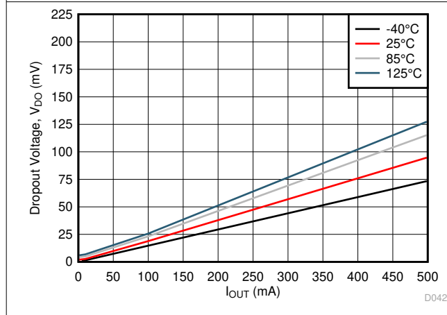
Figure 6-45. LP5912-3.3 Dropout Voltage ( V_{DO} ) vs I_{OUT}
