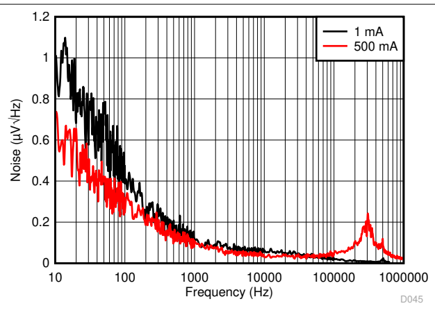
Figure 6-48. LP5912-3.3 Noise vs Frequency
