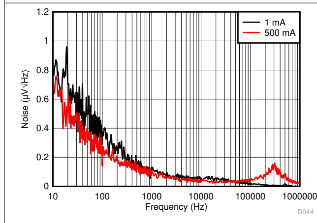
Figure 6-47. LP5912-1.8 Noise vs Frequency
