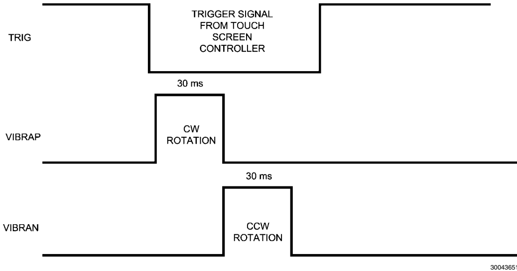
FIGURE 18. Control Waveform
