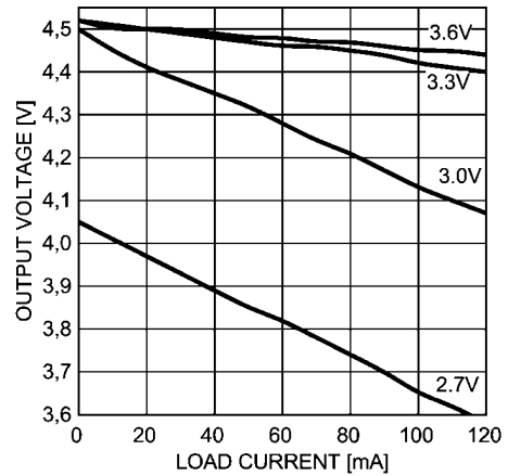
Output Voltage of the Charge Pump (1.5x) as a Function of Load Current at Four Input Voltage Levels
