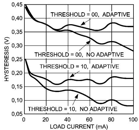
Effect of Adaptive Hysteresis on the Width of the Hysteresis Loop; Load = 6 x Nichia NSCW100 WLEDs on D1 to D6 @ 100% PWM
