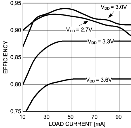
Charge Pump 1.5x Efficiency vs Load Current
