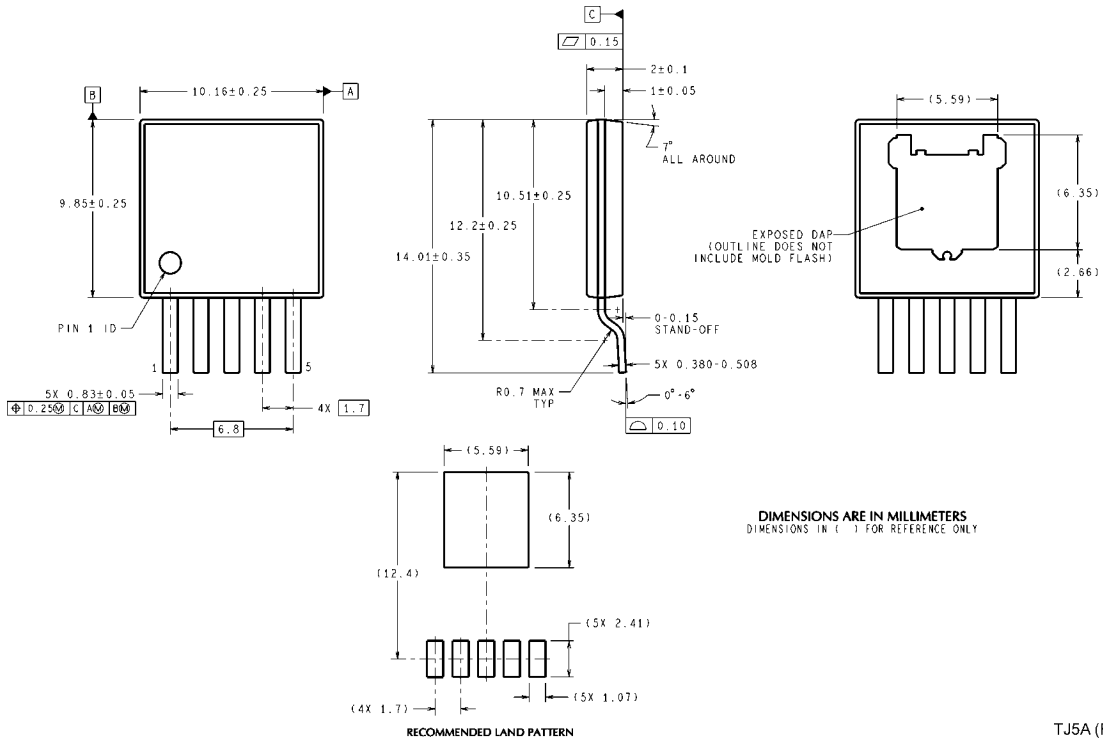
TO-263 THIN, 5 Lead, Molded, 1.7mm Pitch, Surface Mount NS Package Number TJ5A
