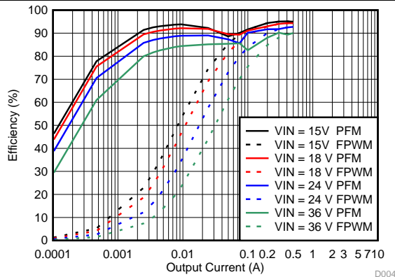
Figure 19. Efficiency
