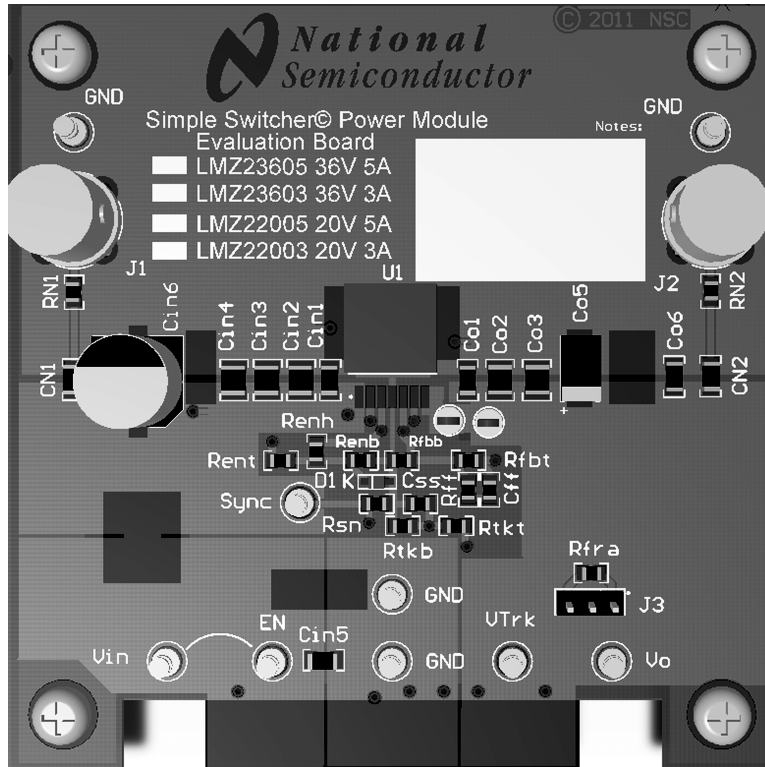
Figure 53. Top View Evaluation Board – See SNVA457
