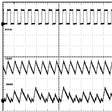
Figure 51. CCM and DCM Operating Modes
