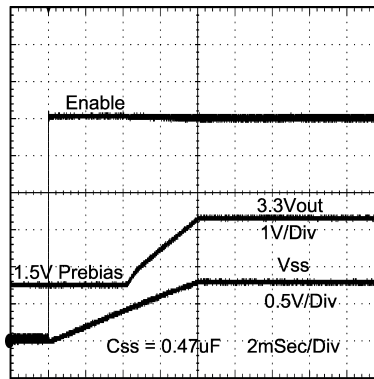
Figure 50. Pre-Biased Startup
