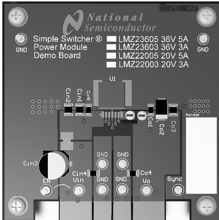
Figure 54. Top View Demonstration Board – See SNVA473
