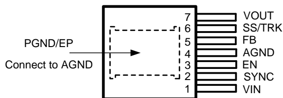
Figure 2. Top View – 7-Lead PFM
