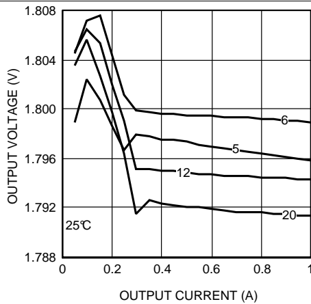
Figure 25. Line and Load Regulation at 25°C
