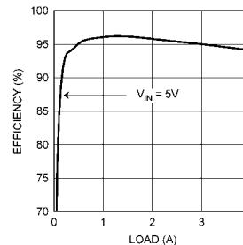
Efficiency ( V_{OUT} = 3.3V )
