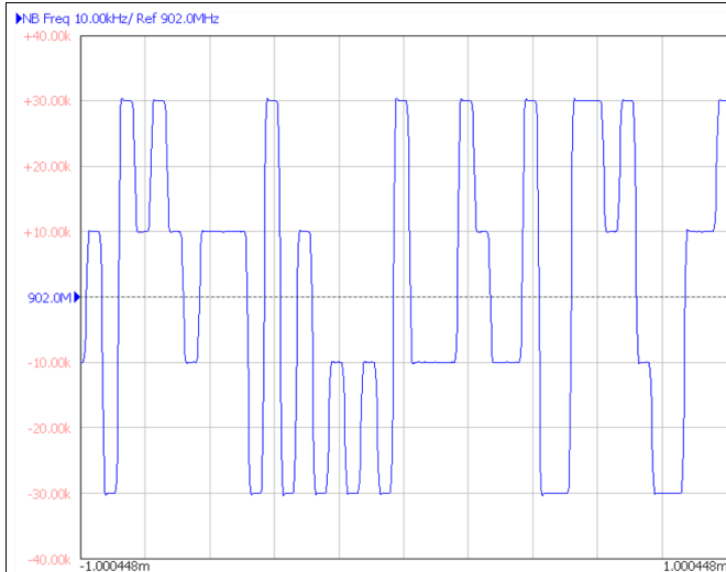
Figure 70. 4FSK Modulation
