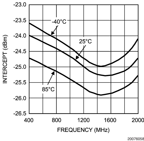
Logarithmic Intercept vs. Frequency (LMV226)
