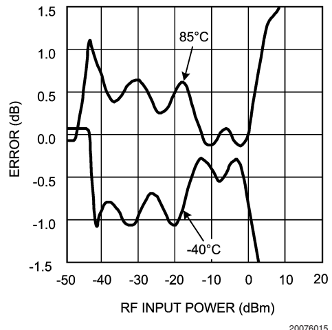
Output Variation vs. RF Input Power Normalized to 25^\circ C @ 2000 MHz (LMV228)
