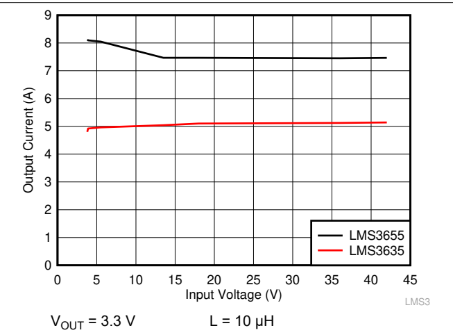
Figure 9-26. Output Current Level for Overcurrent Protection Trip
