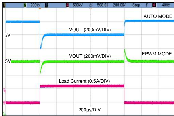
LMR36506MSC5 V_{OUT} = 5V Fixed 2.2 MHz 0 A to 0.6 A, 1 A/µs
