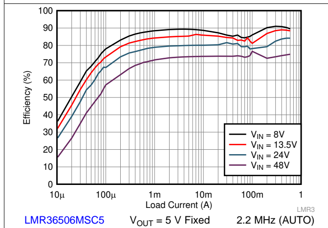
Figure 35. Efficiency
