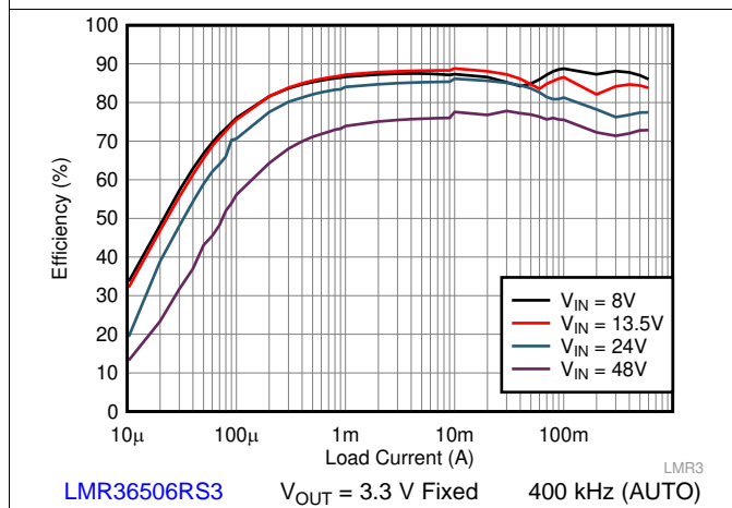
Figure 37. Efficiency
