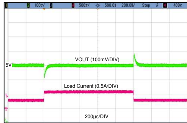
LMR36506MSC5 V_{OUT} = 5V Fixed 2.2 MHz 0.3 A to 0.6 A, 1 A/µs
