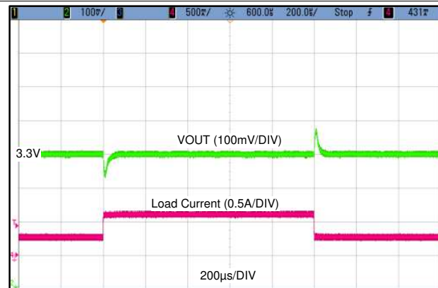
LMR36506RS3 V_{OUT} = 3.3V Fixed 400 kHz 0.3 A to 0.6 A, 1 A/µs
