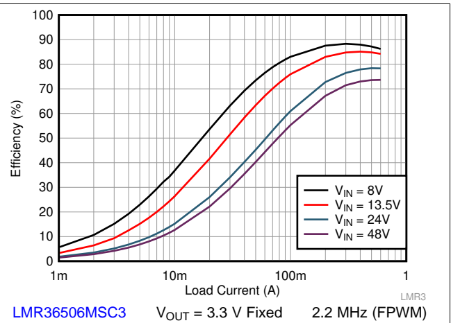
Figure 34. Efficiency
