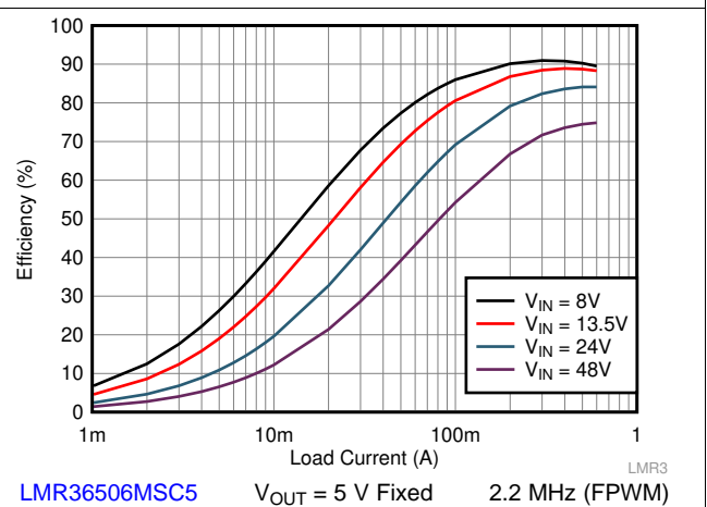
Figure 36. Efficiency
