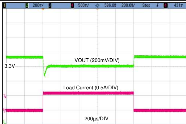
LMR36506RS3 V_{OUT} = 3.3V Fixed 400 kHz 0 A to 0.6 A, 1 A/µs
