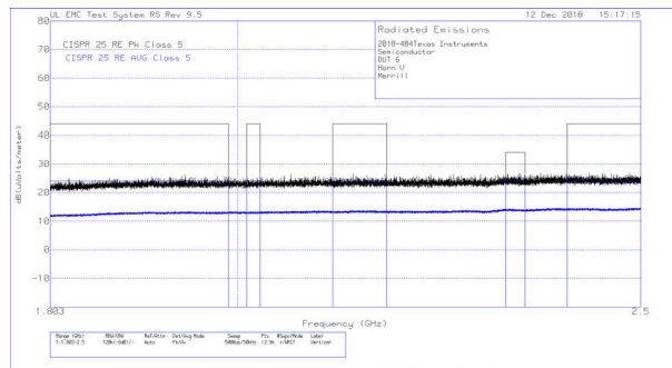
Figure 10-23. Radiated EMI Log Log Vertical vs. CISPR25 Limits
