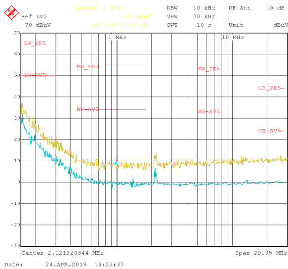
V_{IN} = 13.5\text{ V} V_{OUT} = 5\text{ V} I_{OUT} = 1.5\text{ A} Frequency Tested: 150 kHz to 30 MHz
