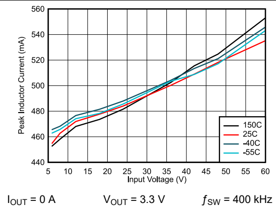
Figure 8-6. I_{PEAK-MIN}
