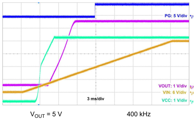
Figure 10-14. Start-Up Waveform
