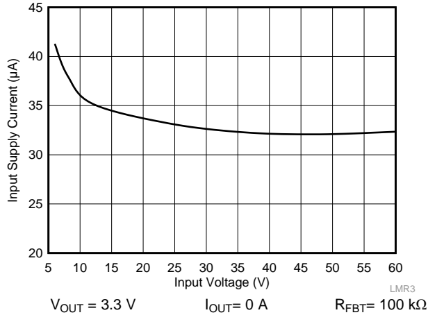
Figure 26. Input Supply Current
