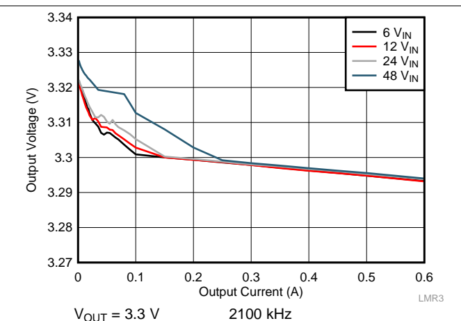
Figure 35. Load Regulation
