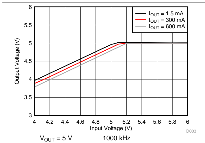
Figure 24. Overall Dropout Characteristic
