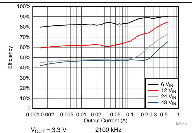
Figure 33. Efficiency
