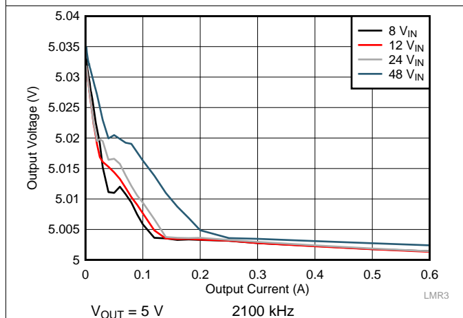
Figure 34. Load Regulation
