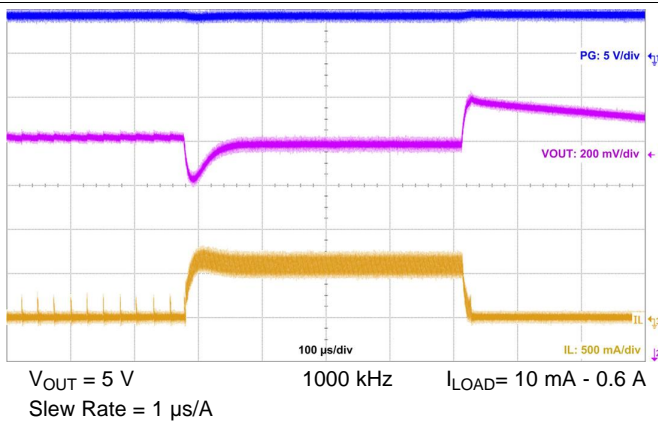
Figure 30. Load Transient
