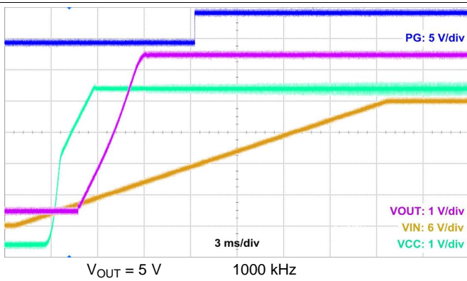
Figure 28. Start-Up Waveform
