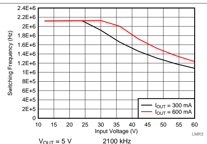
Figure 37. Switching Frequency vs Input Voltage
