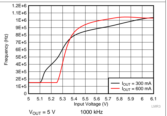
Figure 25. Frequency Dropout Characteristic
