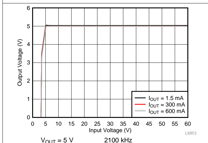
Figure 36. Line Regulation
