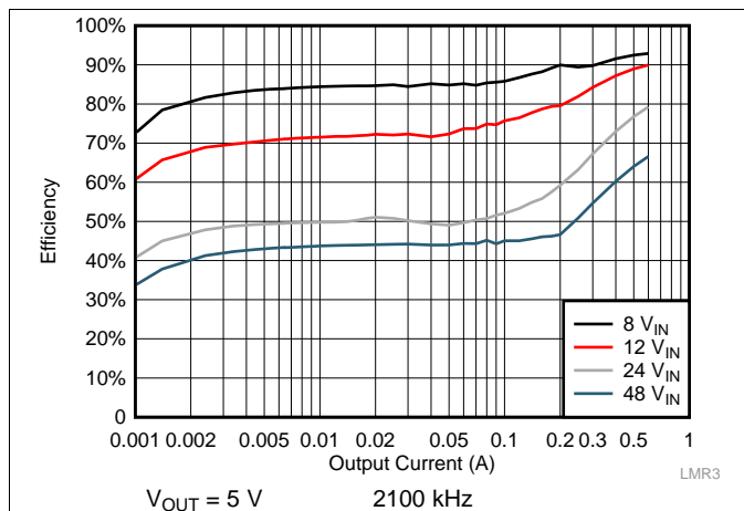
Figure 32. Efficiency
