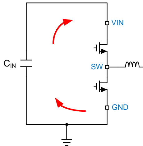
Figure 45. Current Loops with Fast Edges
