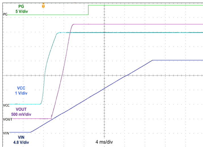
Figure 11. Typical Start-up Behavior V_{IN} = 24\text{ V} , V_{OUT} = 3.3\text{ V} , I_{OUT} = 0.6\text{ A}
