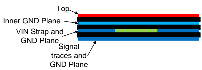
Figure 46. Example Layout
