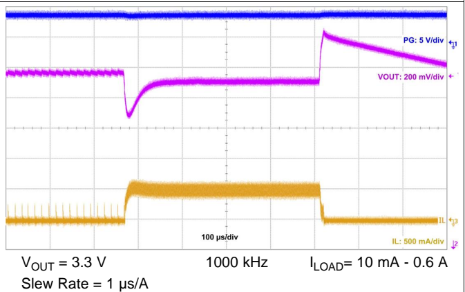
Figure 31. Load Transient
