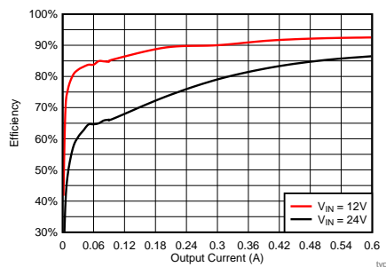
Efficiency vs Output Current \text{V}_{\text{OUT}} = 5\text{ V} , 1 MHz
