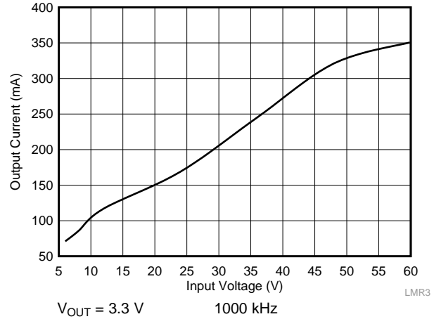
Figure 27. Mode Change Thresholds
