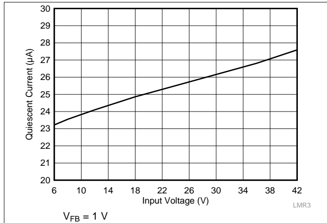
Figure 2. Non-Switching Input Supply Current
