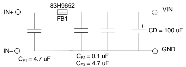
Figure 37. Recommended Input EMI Filter
