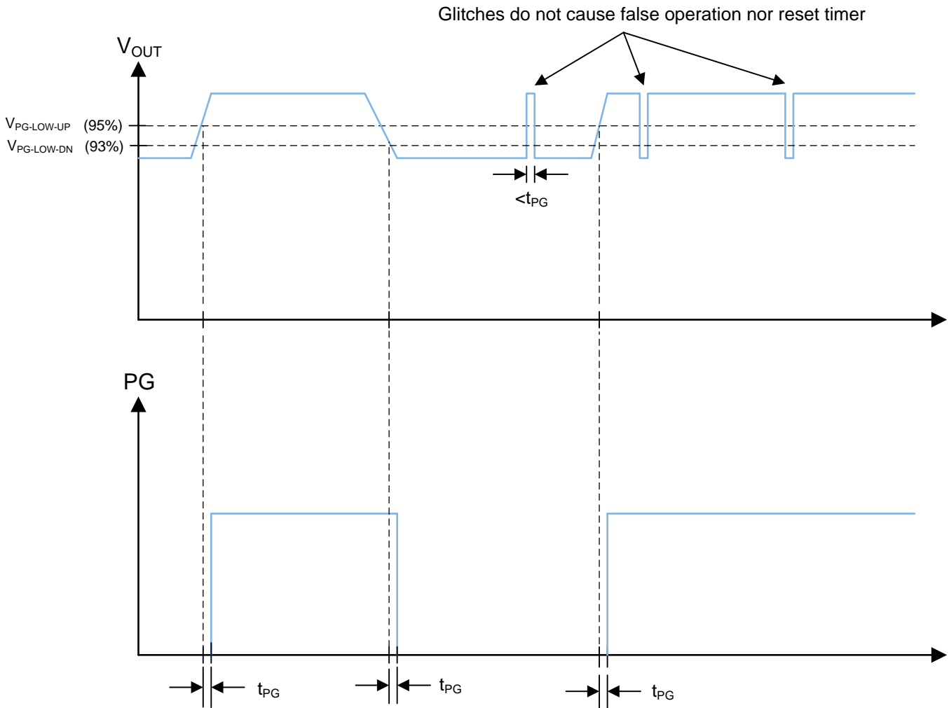
Figure 10. Power-Good-Timing Behavior
