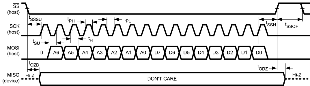
FIGURE 2. SPI Write
