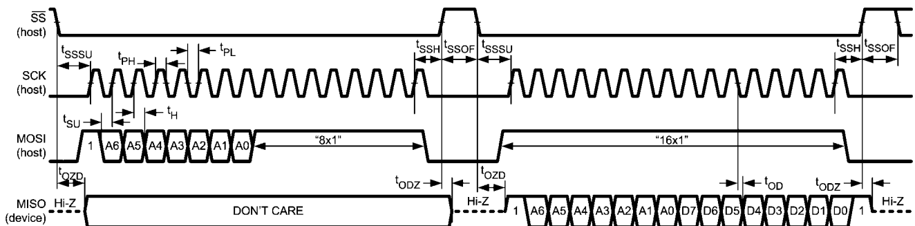
FIGURE 3. SPI Read
