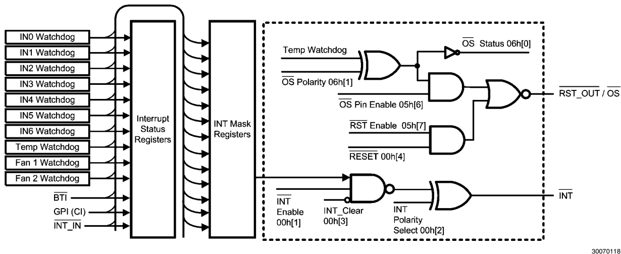
FIGURE 8. Interrupt Structure
