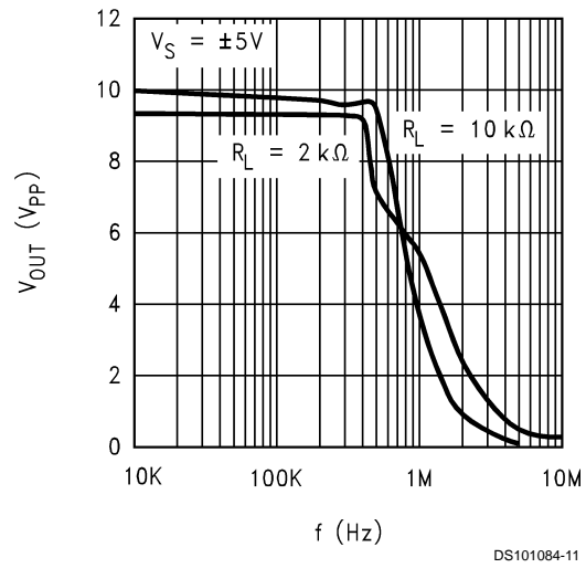
Max Output Swing vs. Frequency
