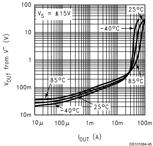
Output Voltage vs. Output Sinking Current
