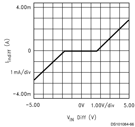
FIGURE 2. Input Stage Current vs Differential Input Voltage
