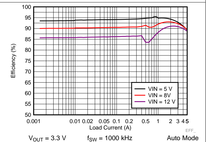
Figure 32. LM73605 Efficiency
