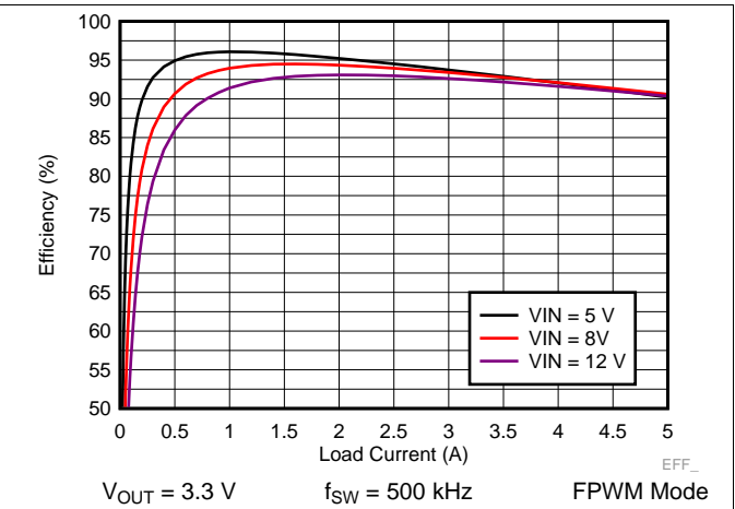
Figure 28. LM73605 Efficiency
