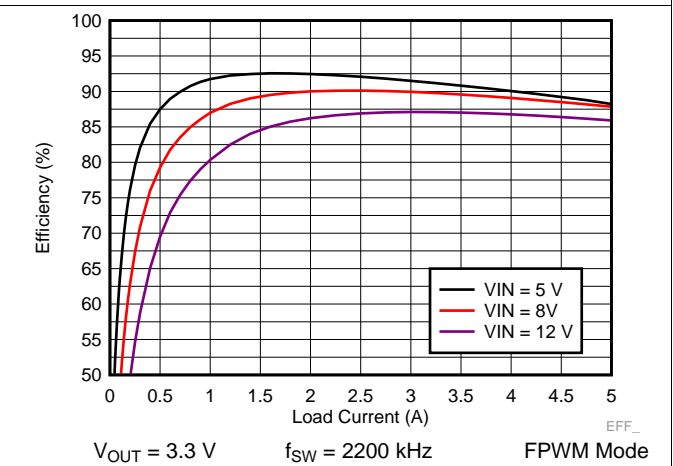
Figure 30. LM73605 Efficiency
