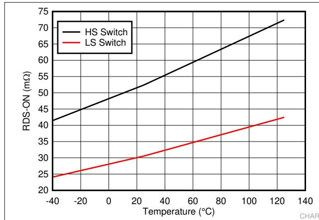
Figure 7-1. High-Side and Low-Side Switches R_{DS-ON}
