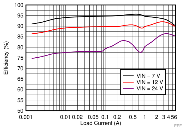
Figure 9-15. LM73606-Q1 Efficiency
