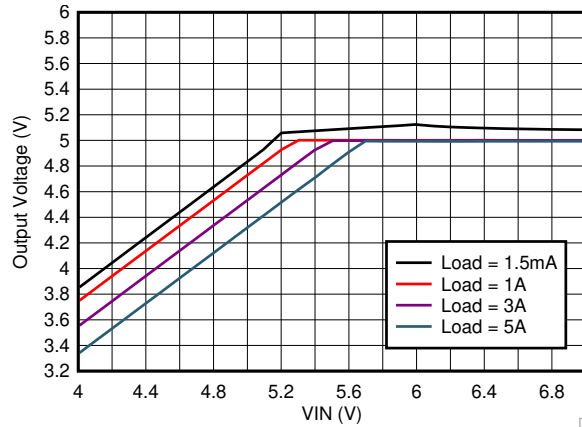
Figure 9-40. LM73605-Q1 Dropout Curve
