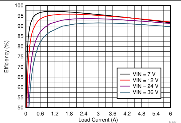
Figure 9-12. LM73606-Q1 Efficiency
