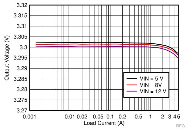
Figure 9-28. LM73606-Q1 Load and Line Regulation
