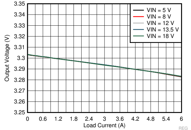
Figure 9-28. LM73606-Q1 Load and Line Regulation
