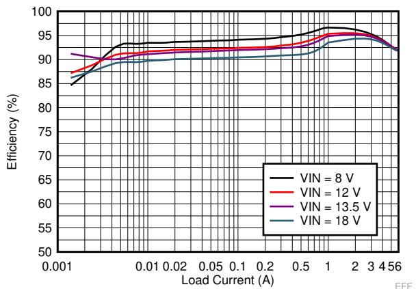
Figure 9-9. LM73605-Q1 Efficiency
