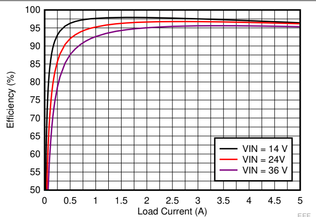
Figure 9-18. LM73606-Q1 Efficiency
