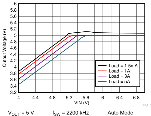
Figure 9-37. LM73605-Q1 Dropout Curve
