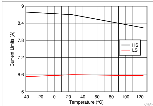
Figure 7-5. LM73605-Q1 High-Side and Low-Side Current Limit
