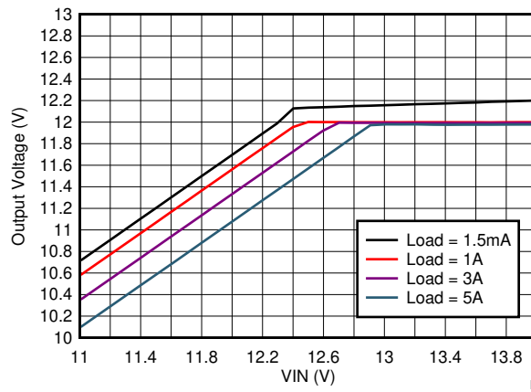
Figure 9-42. LM73606-Q1 Dropout Curve
