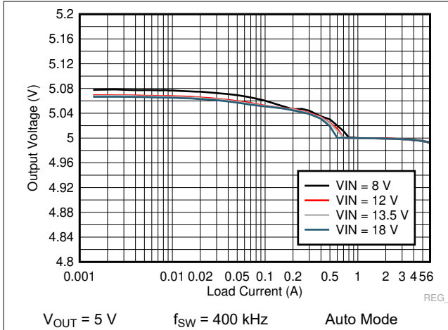
Figure 9-21. LM73606-Q1 Load and Line Regulation
