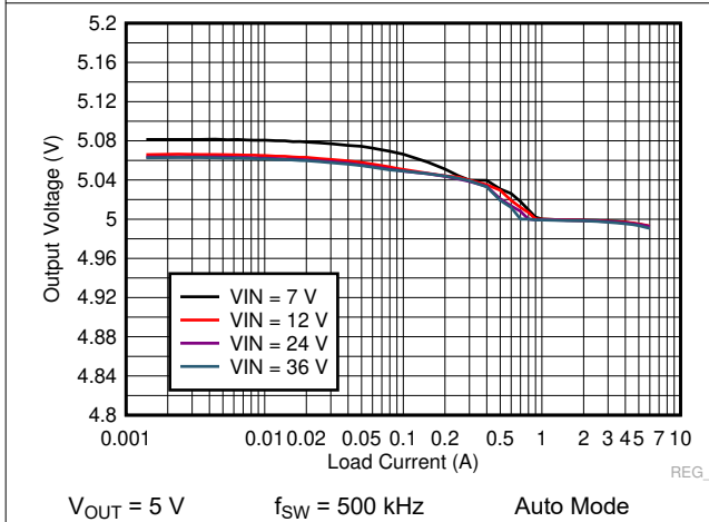
Figure 9-23. LM73606-Q1 Load and Line Regulation
