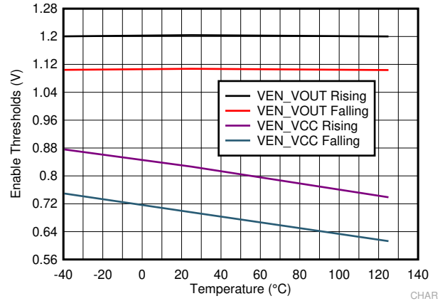
Figure 7-8. Enable Thresholds
