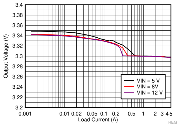
Figure 9-29. LM73605-Q1 Load and Line Regulation
