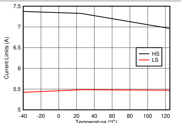
Figure 7-4. LM73605-Q1 High-Side and Low-Side Current Limits
