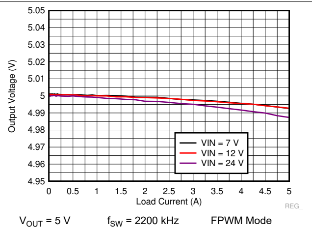
Figure 9-26. LM73605-Q1 Load and Line Regulation
