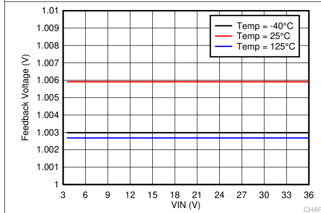
Figure 7-3. Feedback Voltage
