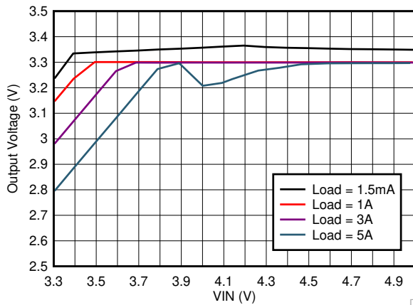
Figure 9-41. LM73606-Q1 Dropout Curve
