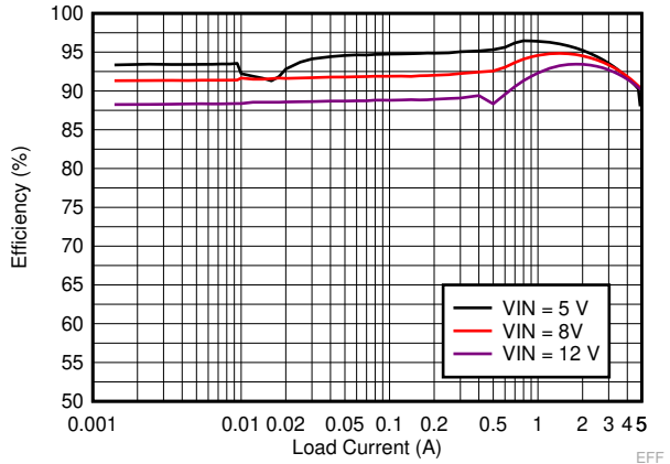
Figure 9-9. LM73605-Q1 Efficiency
