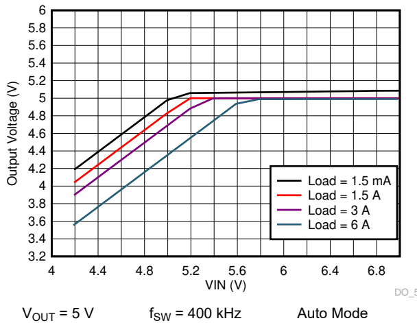
Figure 9-35. LM73606-Q1 Dropout Curve
