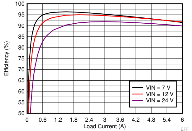
Figure 9-16. LM73606-Q1 Efficiency
