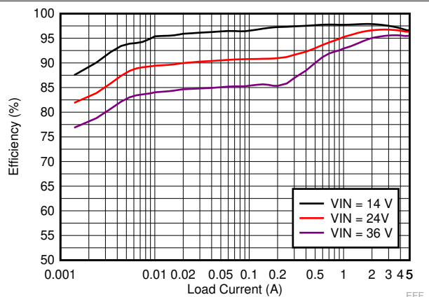
Figure 9-17. LM73606-Q1 Efficiency
