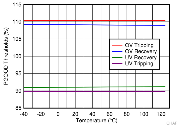
Figure 7-9. PGOOD Thresholds
