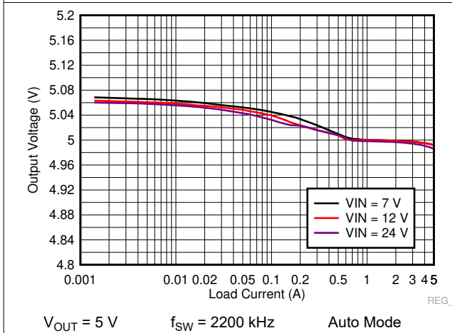
Figure 9-25. LM73605-Q1 Load and Line Regulation
