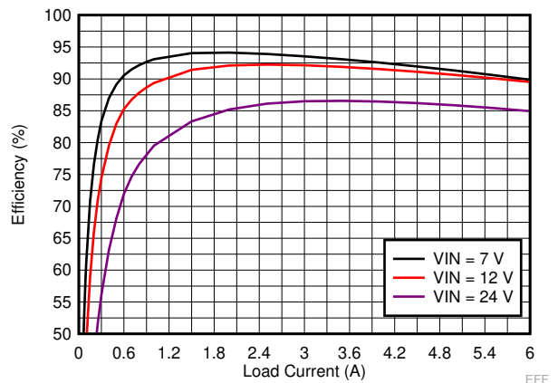
Figure 9-16. LM73606-Q1 Efficiency
