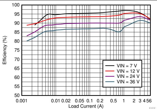
Figure 9-11. LM73606-Q1 Efficiency
