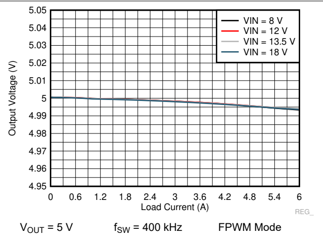
Figure 9-22. LM73606-Q1 Load and Line Regulation
