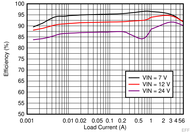
Figure 9-15. LM73606-Q1 Efficiency
