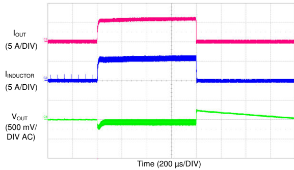
Figure 9-57. LM73606-Q1 Load Transients
