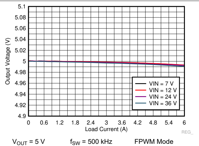
Figure 9-24. LM73606-Q1 Load and Line Regulation
