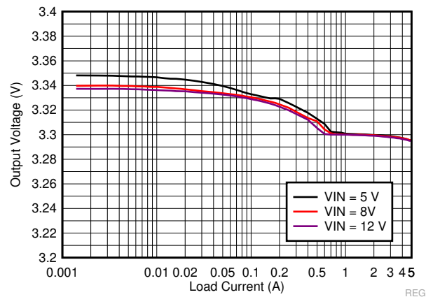
Figure 9-30. LM73605-Q1 Load and Line Regulation
