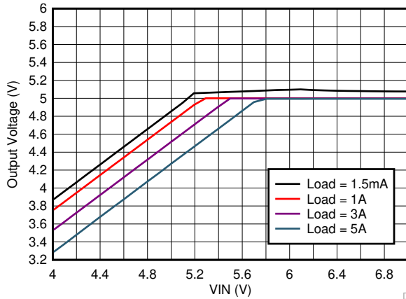
Figure 9-39. LM73605-Q1 Dropout Curve
