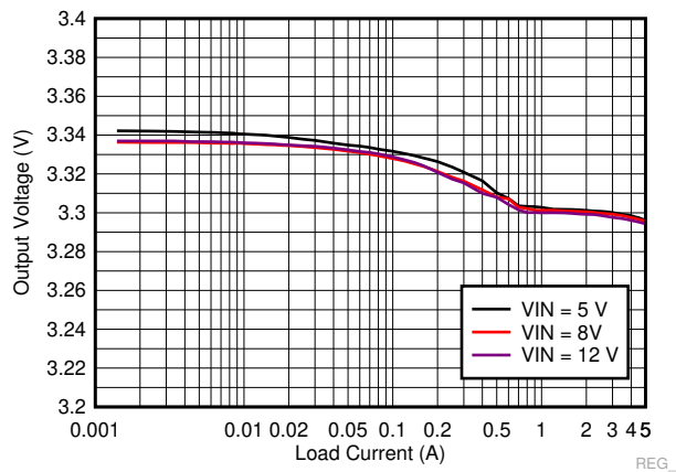
Figure 9-27. LM73606-Q1 Load and Line Regulation
