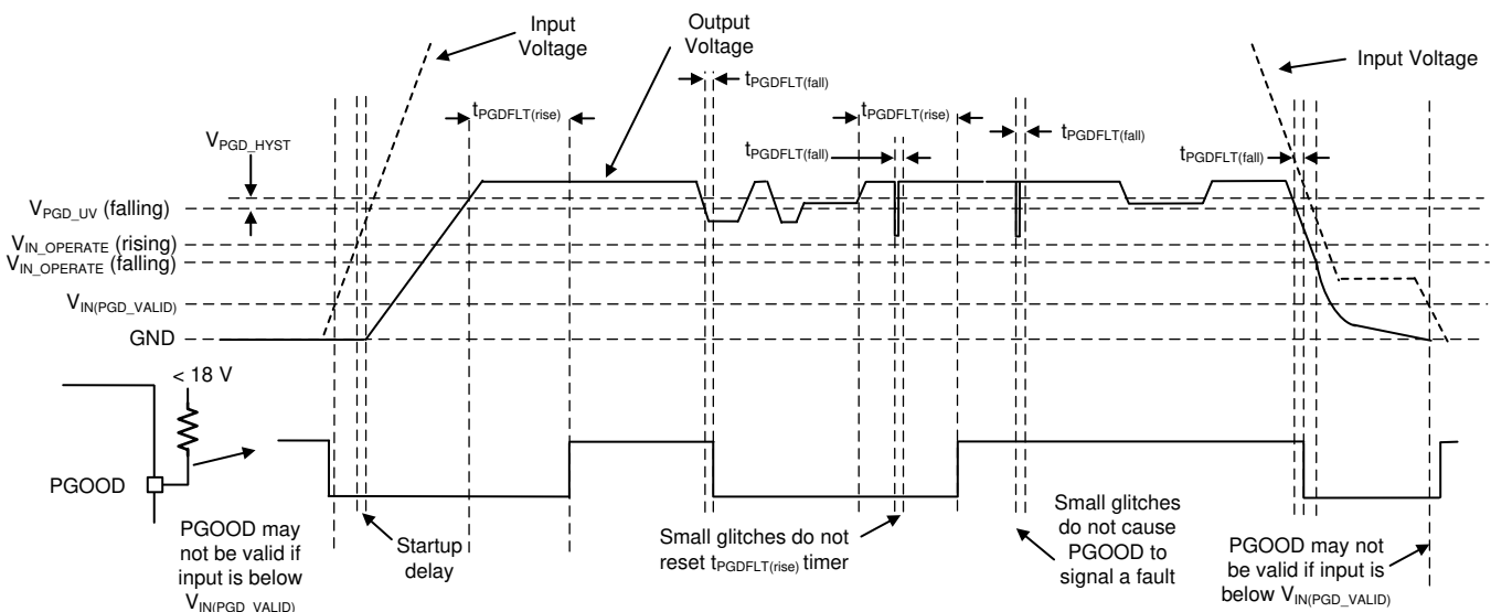
Figure 21. PGOOD Timing Diagram (Excludes OV Events)
