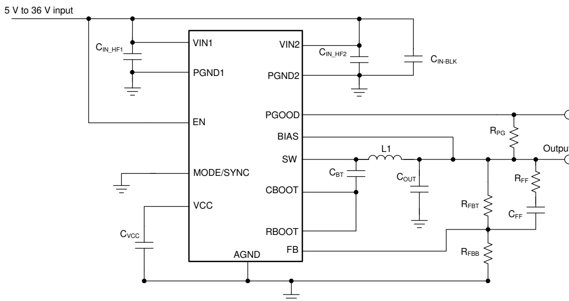
Figure 36. Example Application Circuit
