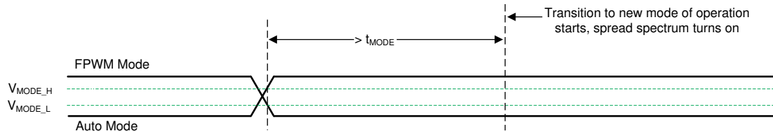
Figure 13. Transition from Auto Mode and FPWM Mode
