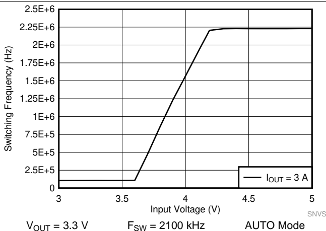
Figure 50. LM62435-Q1 Frequency Dropout Curve
