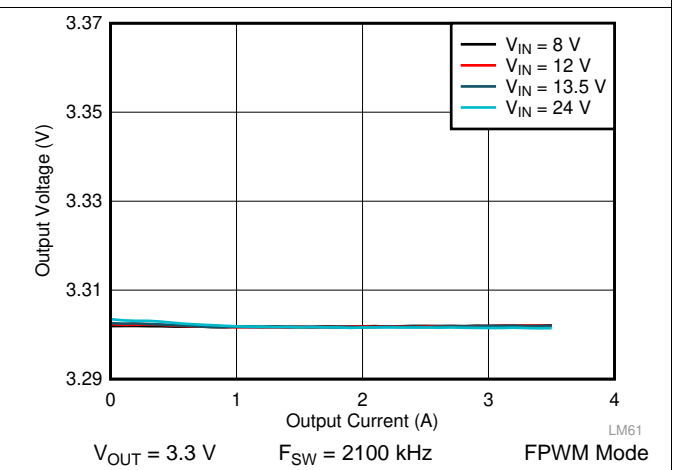
Figure 45. LM62435-Q1 Load and Line Regulation
