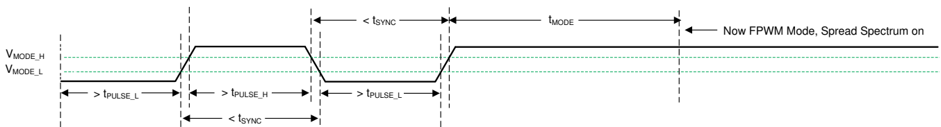
Figure 19. Transition from SYNC Mode to FPWM Mode
