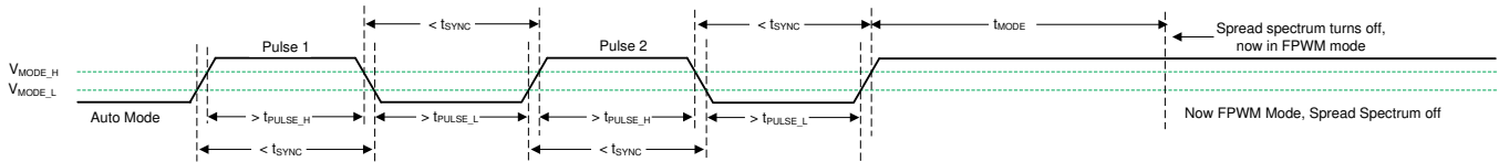
Figure 17. Spread Spectrum Disabled in Transition from Auto Mode to FPWM Mode
