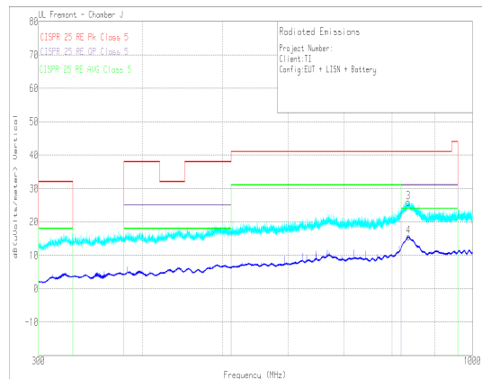
Figure 65. Radiated EMI Log Vertical versus CISPR25 Limits
