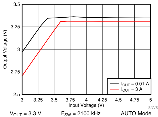
Figure 48. LM62435-Q1 Dropout Curve
