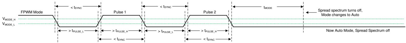
Figure 16. Spread Spectrum Disabled in Transition from FPWM Mode to Auto Mode
