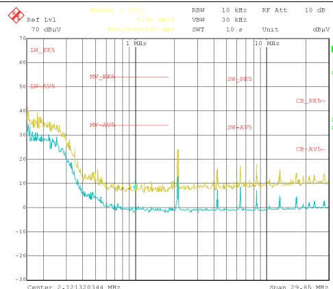
Figure 66. Radiated EMI Log Horizontal versus CISPR25 Limits
