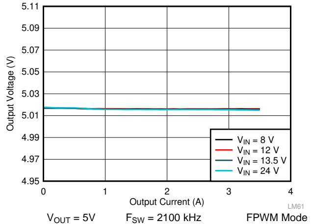
Figure 47. LM62435-Q1 Load and Line Regulation
