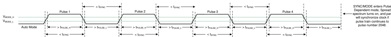
Figure 12. Transition from Auto Mode to Pulse-Dependent Control
