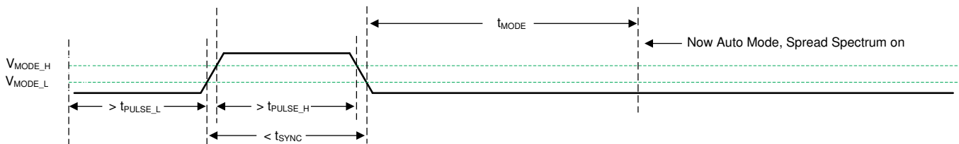
Figure 18. Transition from SYNC Mode to Auto Mode
