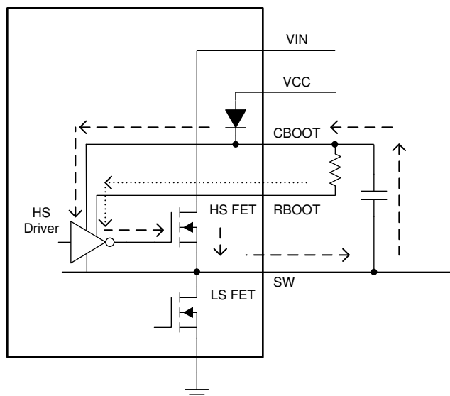
Figure 22. Simplified Circuit Showing How RBOOT Functions
