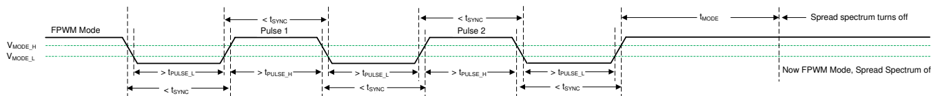
Figure 14. Spread Spectrum Disabled in FPWM Mode
