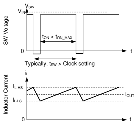
Figure 26. Current Limit Waveforms
