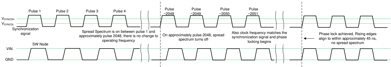
Pulses four and synchronization signal is detected. After the pulse, approximately 2048 ready to synchronize and frequency is adjusted using a glitch free technique. Later, phase is locked.
