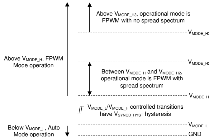
Figure 10. Level-Dependent Mode Selection Settings
