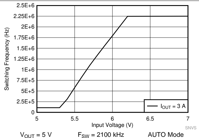
Figure 51. LM62435-Q1 Frequency Dropout Curve
