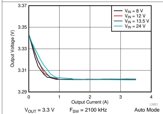
Figure 44. LM62435-Q1 Load and Line Regulation
