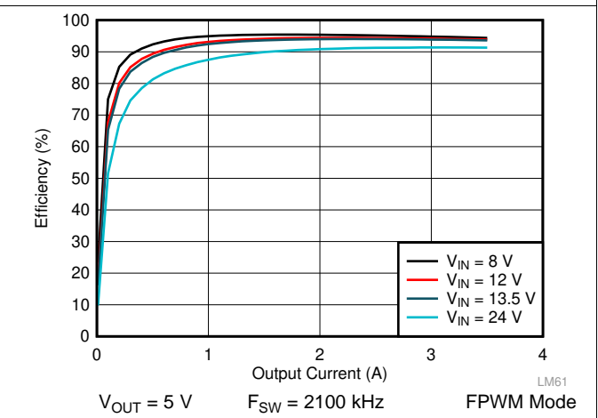
Figure 43. LM62435-Q1 Efficiency
