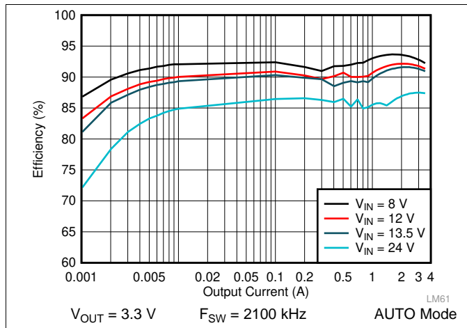
Figure 40. LM62435-Q1 Efficiency
