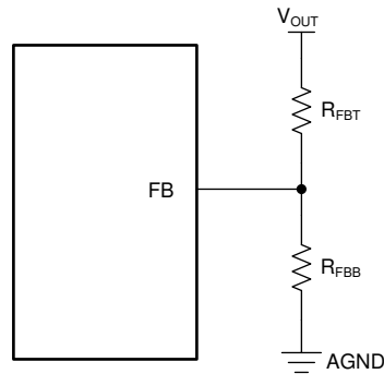
Figure 25. Setting Output Voltage of Adjustable Versions
