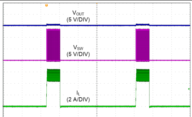
Figure 55. LM62435-Q1 Short Circuit Protection
