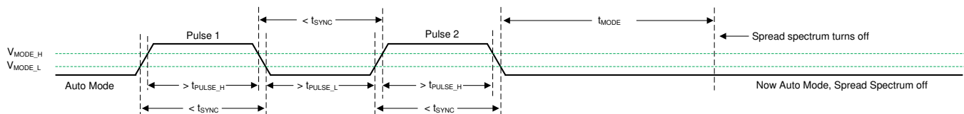
Figure 15. Spread Spectrum Disabled in Auto Mode
