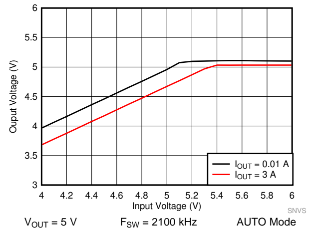
Figure 49. LM62435-Q1 Dropout Curve
