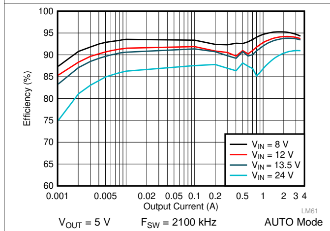
Figure 42. LM62435-Q1 Efficiency
