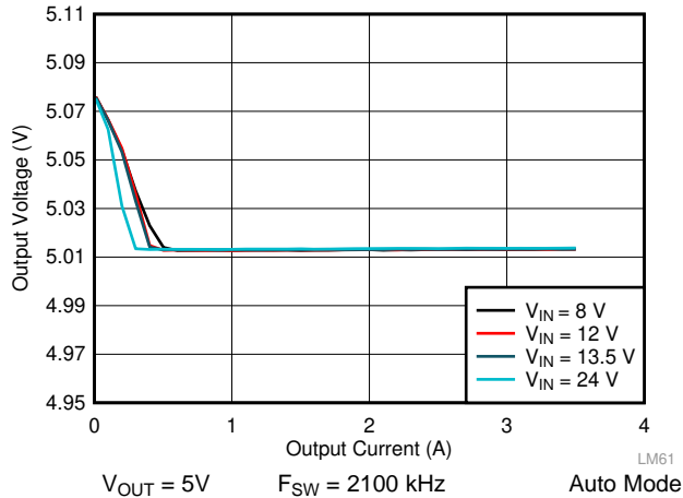
Figure 46. LM62435-Q1 Load and Line Regulation
