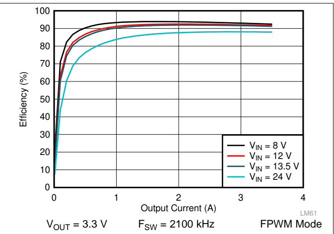
Figure 41. LM62435-Q1 Efficiency
