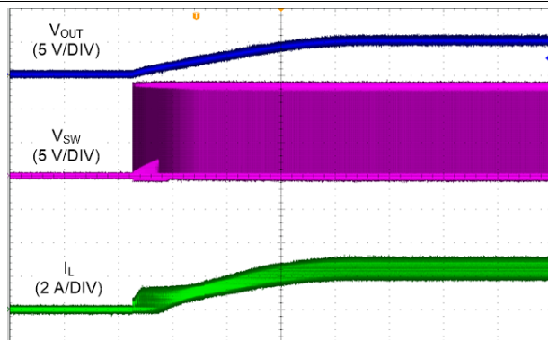
Figure 54. LM62435-Q1 Start-up with 3.25 A
