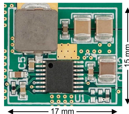
Industrial Power Supply With 5-V, 3-A Output
