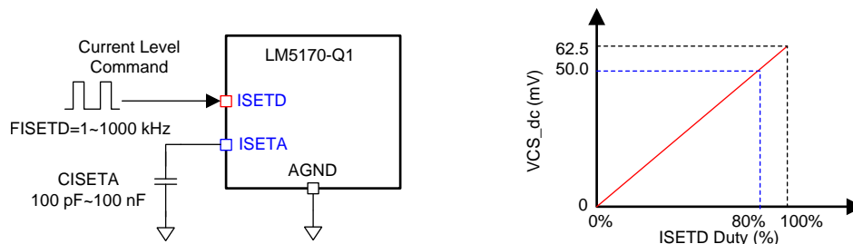
Figure 22. Pin Configurations for Current Setting Using a PWM Signal
