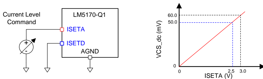
Figure 21. Pin Configurations for Current Setting Using an Analog Voltage Signal
