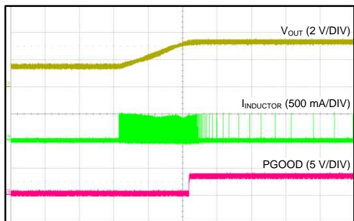
Time (1 ms/DIV)
