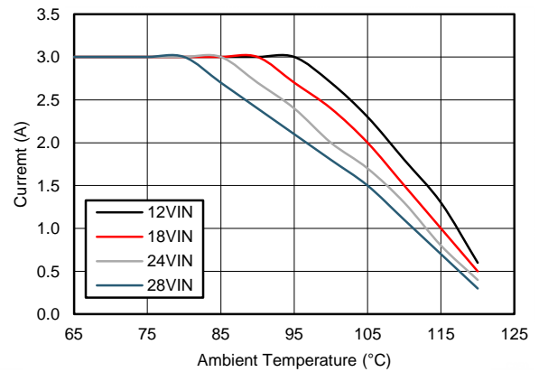
Figure 84. Derating Curve
