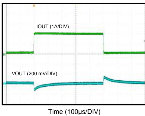
V_{OUT} = 5\text{ V} F_S = 500\text{ kHz}
