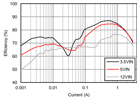
V_{OUT} = 1\text{ V} F_S = 500\text{ kHz}
