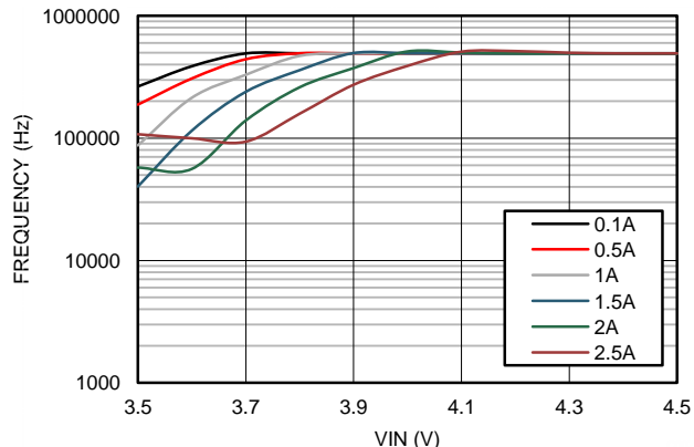
V_{OUT} = 3.3\text{ V} F_S = 500\text{ kHz}
