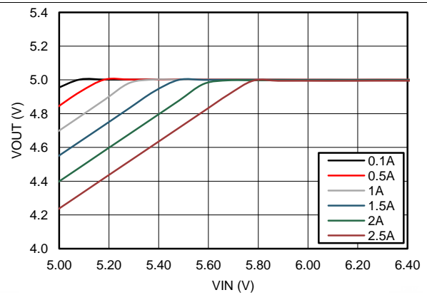
Figure 14. Dropout Curve
