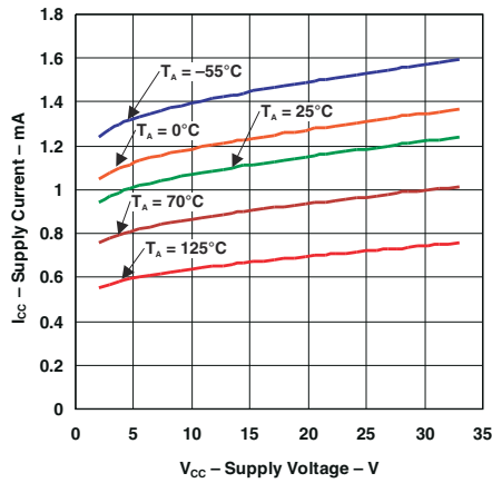
Figure 7-1. Supply Current vs Supply Voltage
