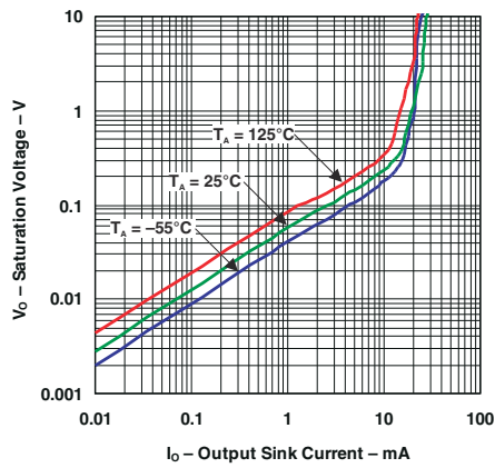
Figure 7-3. Output Saturation Voltage
