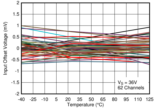
Figure 7-15. Input Offset Voltage vs. Temperature at 36V
