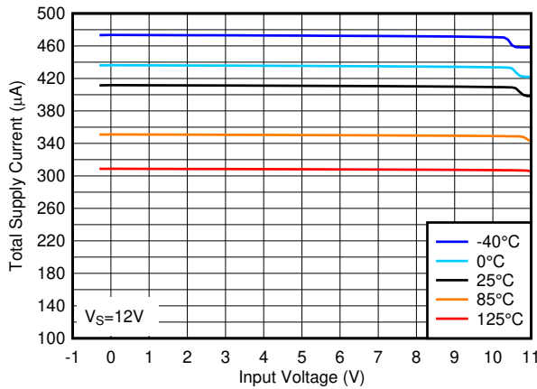
Figure 7-10. Total Supply Current vs. Input Voltage at 12V
