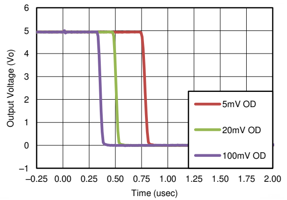
Figure 9-3. Response Time for Various Overdrives (Negative Transition)
