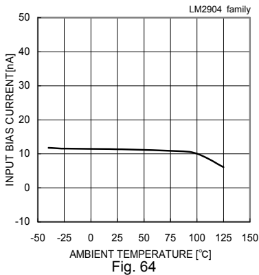
Fig. 64 Input Bias Current – Ambient Temperature (VCC=30[V], Vicm=28[V], VOUT=1.4[V])
