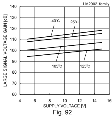
Fig. 92 Large Signal Voltage Gain – Supply Voltage (RL=2[kΩ])
