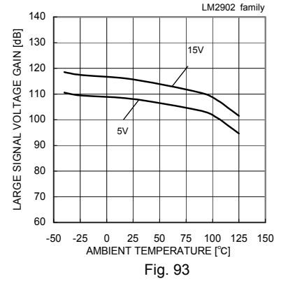
Fig. 93 Large Signal Voltage Gain – Ambient Temperature (RL=2[kΩ])
