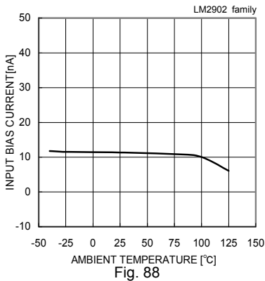
Fig. 88 Input Bias Current – Ambient Temperature (VCC=30[V], Vicm=28[V], VOUT=1.4[V])
