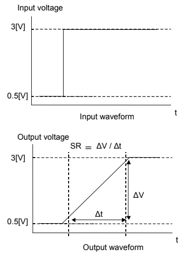
Fig.100 Slew Rate Input Waveform
