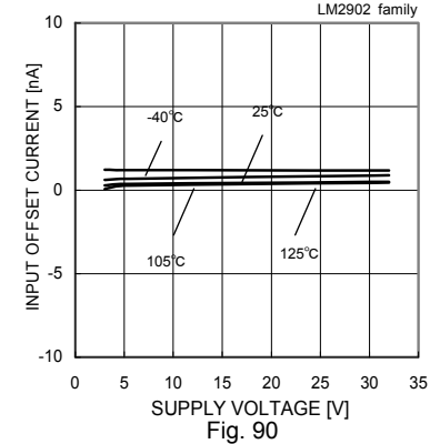
Fig. 90 Input Offset Current – Supply Voltage (Vicm=0[V], VOUT=1.4[V])
