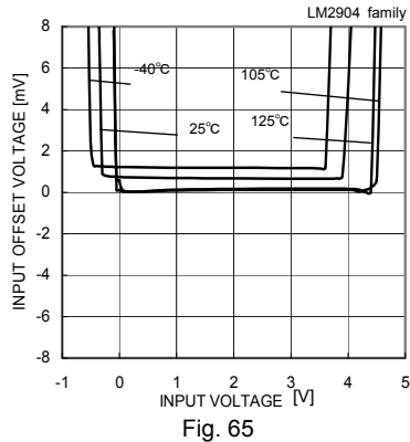
Fig. 65 Input Offset Voltage – Common Mode Input Voltage (VCC=5[V])
