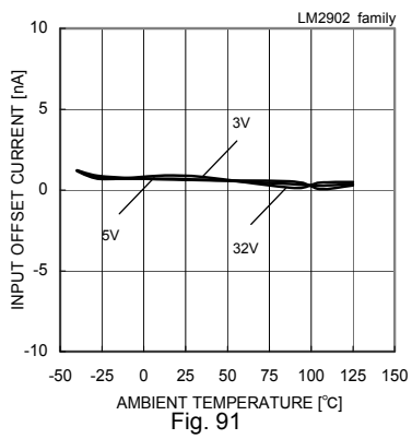
Fig. 91 Input Offset Current – Ambient Temperature (Vicm=0[V], VOUT=1.4[V])
