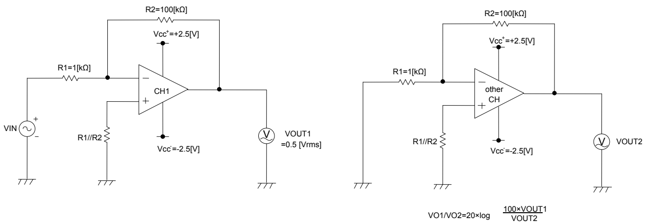
Fig.101 Measurement Circuit3
