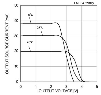
Fig. 30 Output Source Current - Output Voltage ( V_{CC}=5[V] )
