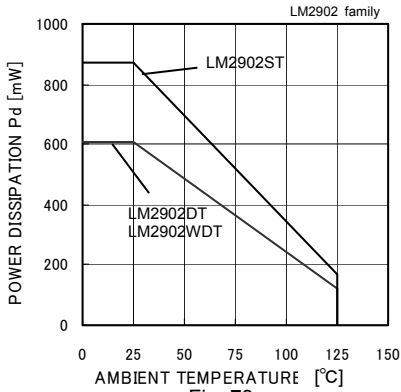
Fig. 73 Derating Curve
