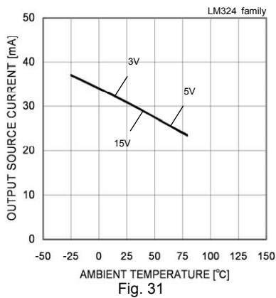
Fig. 31 Output Source Current - Ambient Temperature ( V_{OUT}=0[V] )
