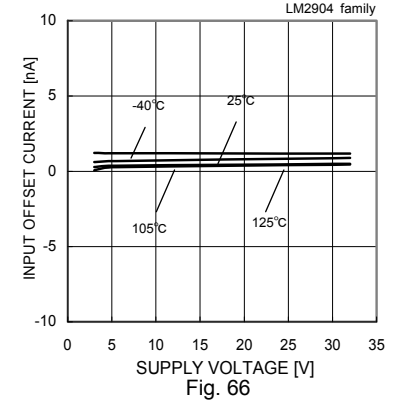
Fig. 66 Input Offset Current – Supply Voltage (Vicm=0[V], VOUT=1.4[V])
