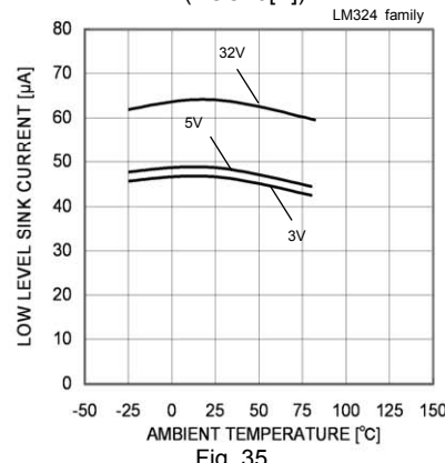
Fig. 35 Low Level Sink Current - Ambient Temperature ( V_{OUT}=0.2[V] )
