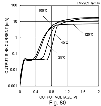
Fig. 80 Output Sink Current - Output Voltage (VCC=5[V])
