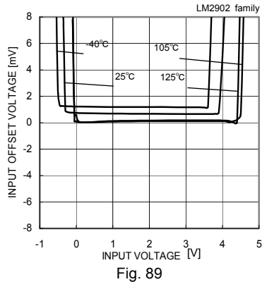
Fig. 89 Input Offset Voltage – Common Mode Input Voltage (VCC=5[V])
