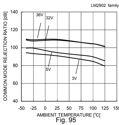
Fig. 95 Common Mode Rejection Ratio – Ambient Temperature
