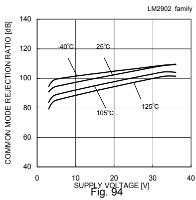
Fig. 94 Common Mode Rejection Ratio – Supply Voltage
