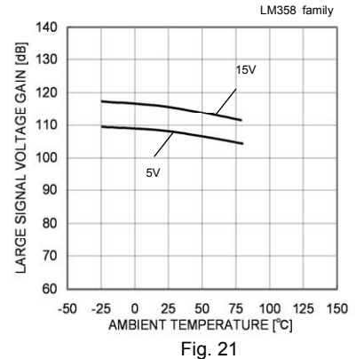
Fig. 21 Large Signal Voltage Gain – Ambient Temperature (RL=2[kΩ])
