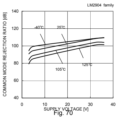
Fig. 70 Common Mode Rejection Ratio – Supply Voltage
