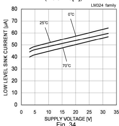
Fig. 34 Low Level Sink Current - Supply Voltage ( V_{OUT}=0.2[V] )
