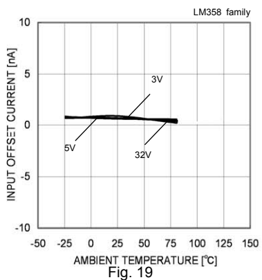
Fig. 19 Input Offset Current – Ambient Temperature (Vicm=0[V], VOUT=1.4[V])
