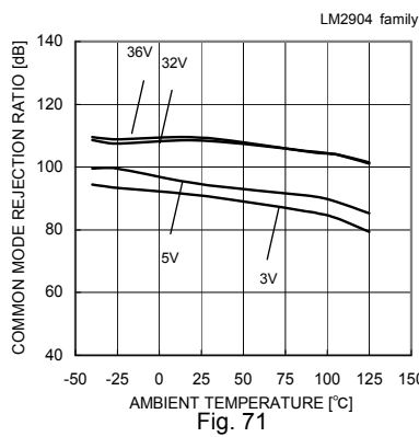
Fig. 71 Common Mode Rejection Ratio – Ambient Temperature
