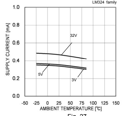
Fig. 27 Supply Current - Ambient Temperature
