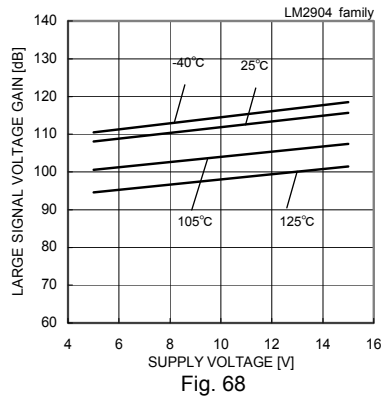
Fig. 68 Large Signal Voltage Gain – Supply Voltage (RL=2[kΩ])
