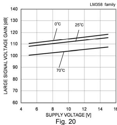
Fig. 20 Large Signal Voltage Gain – Supply Voltage (RL=2[kΩ])
