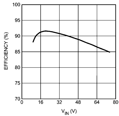
Figure 37. Sample Buck-Boost Efficiency vs Input Voltage. V_o = 21\text{ V}
