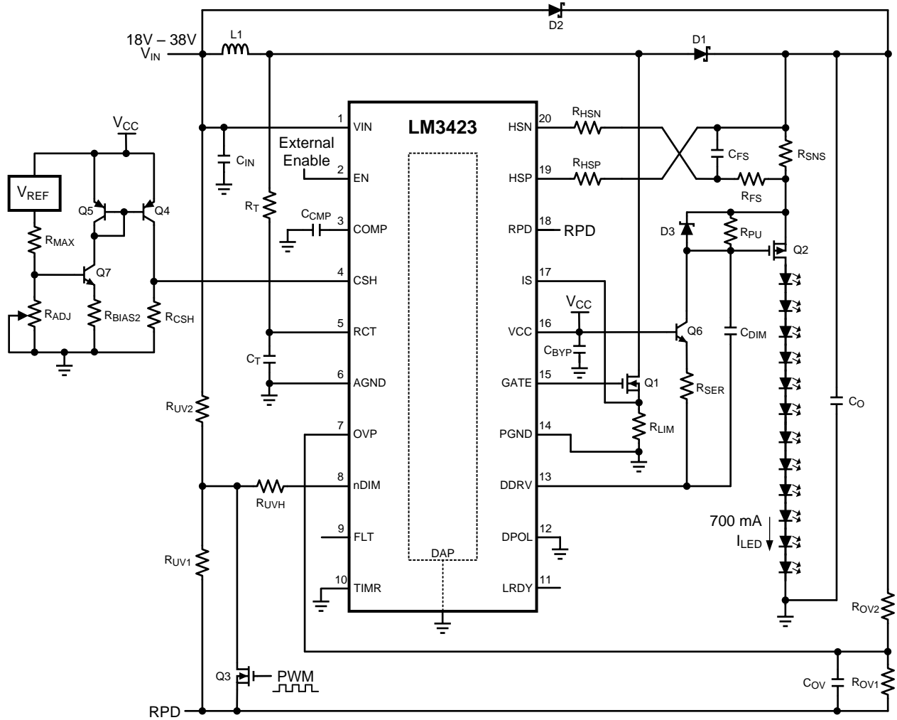
Figure 40. LM3423 Boost Application
