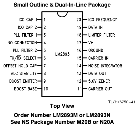
FIGURE 2. Connection Diagrams
