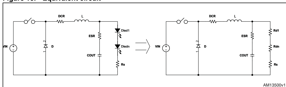
Figure 16. Equivalent circuit
