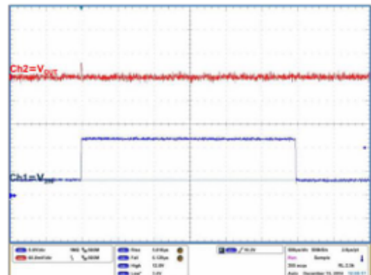
Figure 25. Line transient ( V_{OUT} = 1.2\text{ V} )
