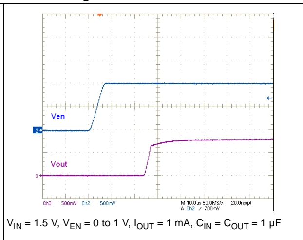
Figure 15. Enable transient
