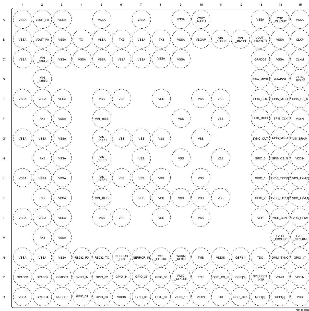
Figure 7-1. Pin Diagram
