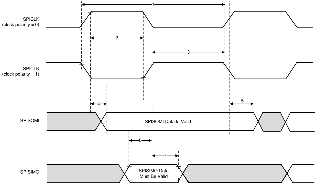
Figure 8-7. SPI Slave Mode External Timing (CLOCK PHASE = 0)
