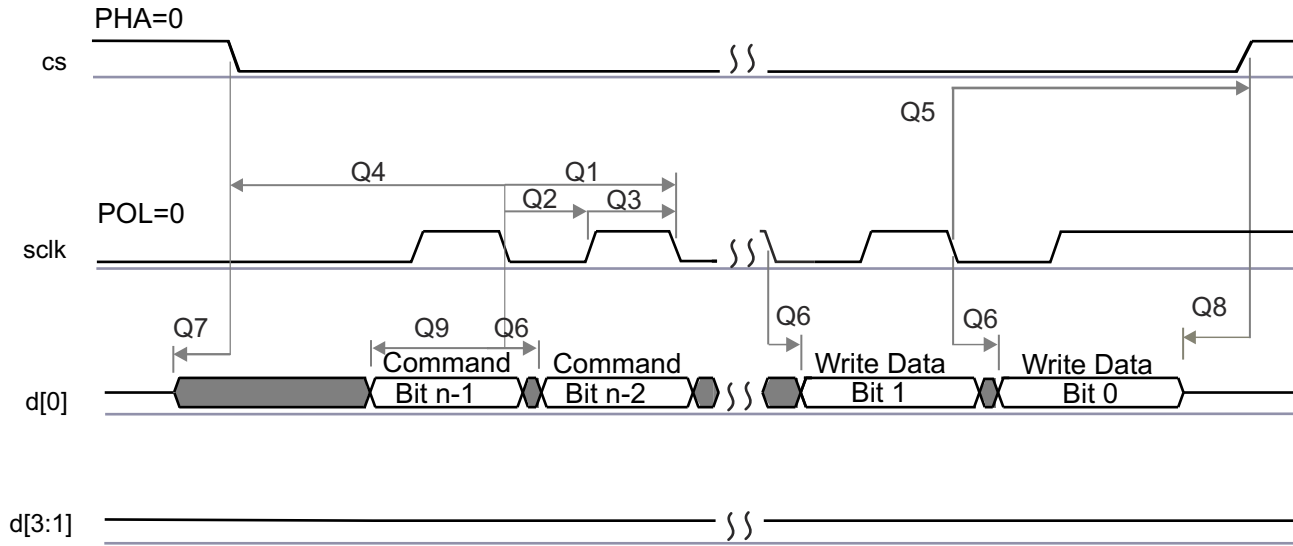
Figure 8-14. QSPI Write (Clock Mode 0)
