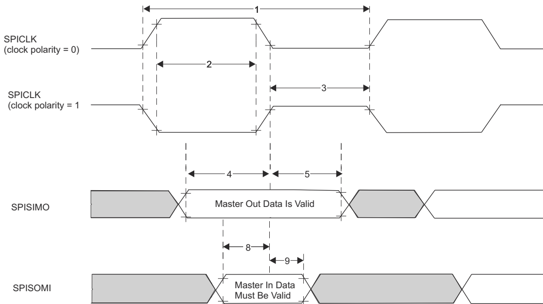
Figure 8-3. SPI Master Mode External Timing (CLOCK PHASE = 0)
