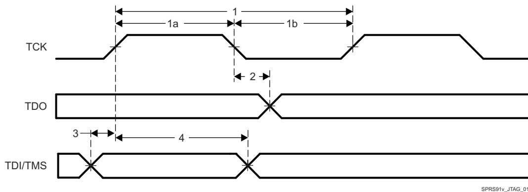
Figure 8-19. JTAG Timing
