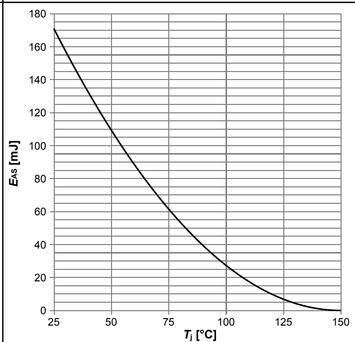
Diagram 12: Avalanche energy
