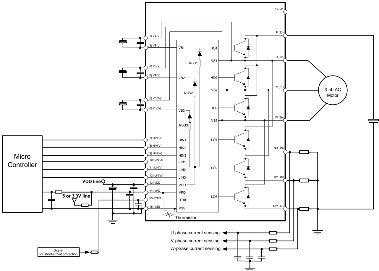
Figure 9: Application circuit
