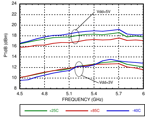
P1dB vs. Temperature [1] [2]
