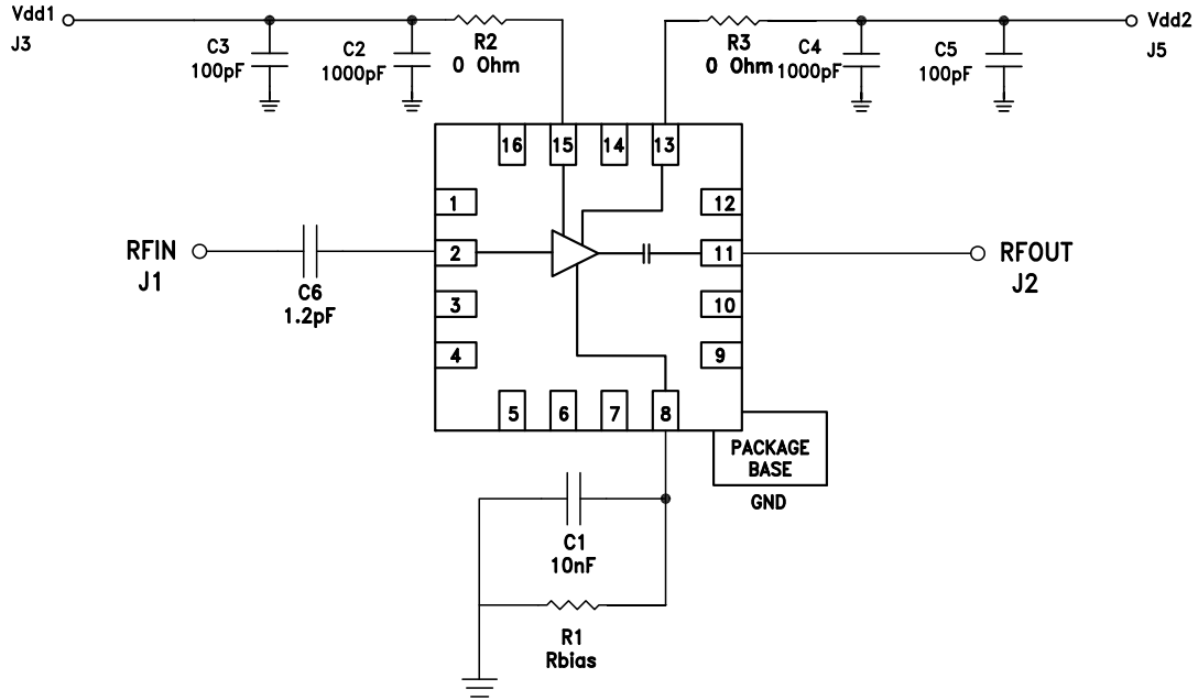
HMC717ALP3FE Evaluation Board Schematic
