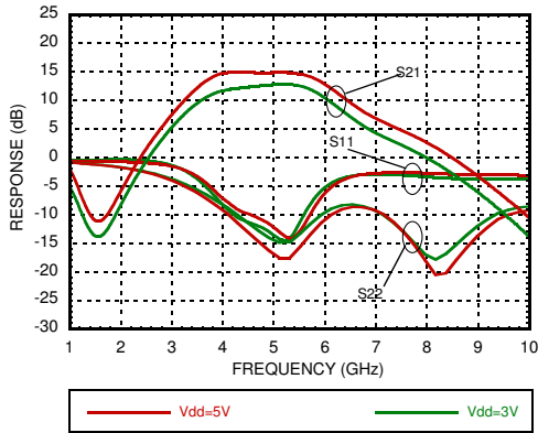
Broadband Gain & Return Loss [1][2]
