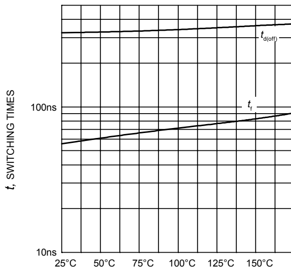
Figure 11. Typical switching times as a function of junction temperature (inductive load, V_{CE}=600\text{V} , V_{GE}=0/15\text{V} , I_C=25\text{A} , R_G=10\Omega , Dynamic test circuit in Figure E)
